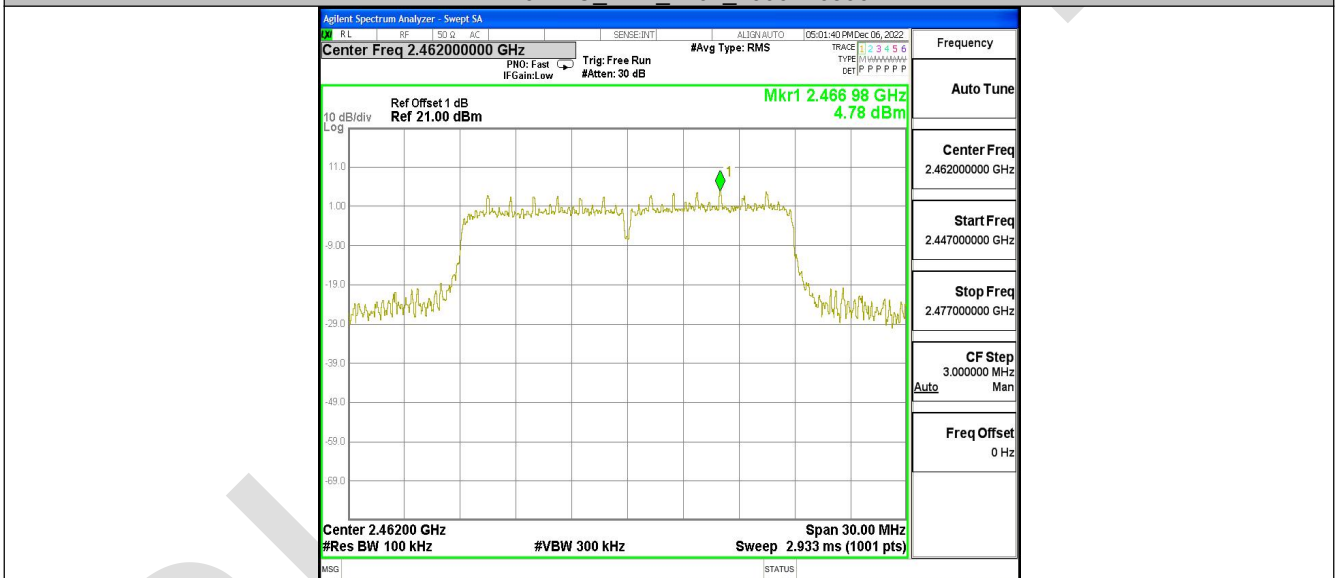
11N20SISO_Ant2_2462_0~Reference
