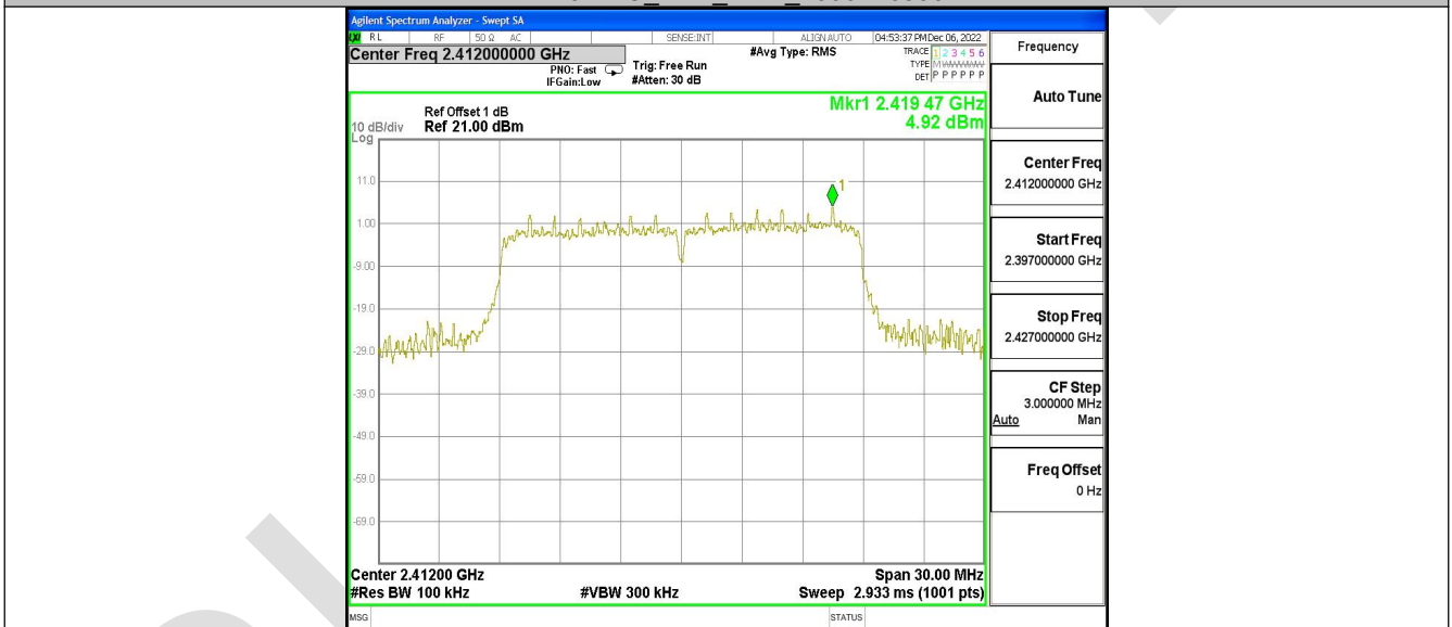
11N20SISO_Ant2_2412_0~Reference
