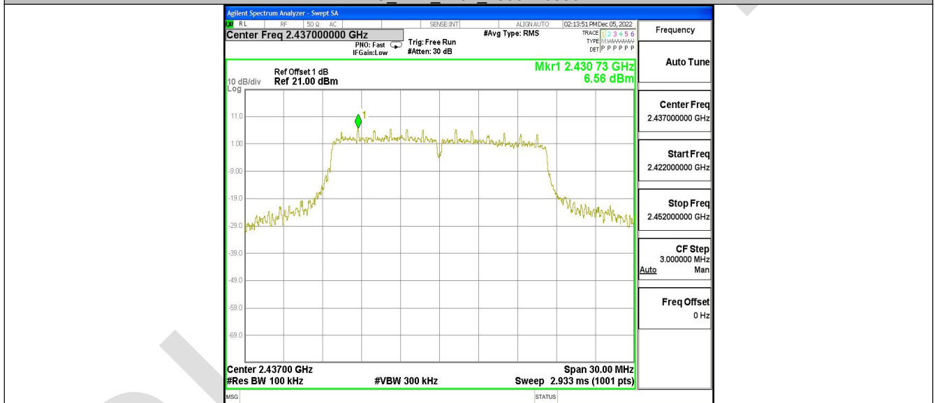
11G_Ant2_2437_0~Reference
