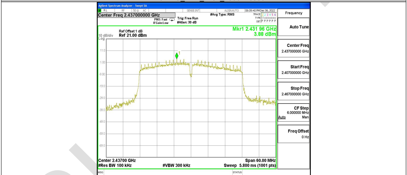
11N40SISO_Ant2_2437_0~Reference
