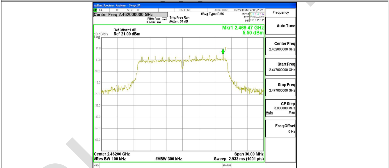
11G_Ant2_2462_0~Reference
