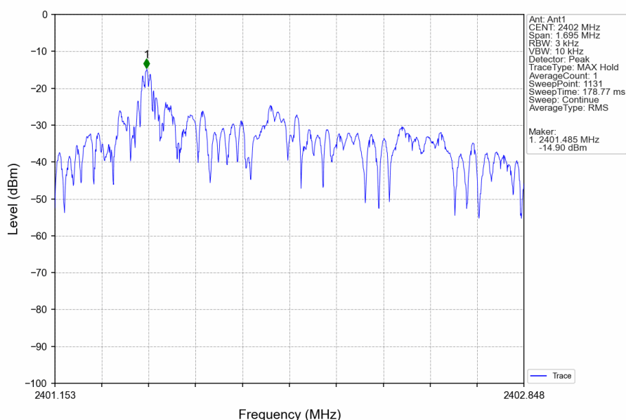
2M_LCH_2402MHz_Ant1_NTNV
