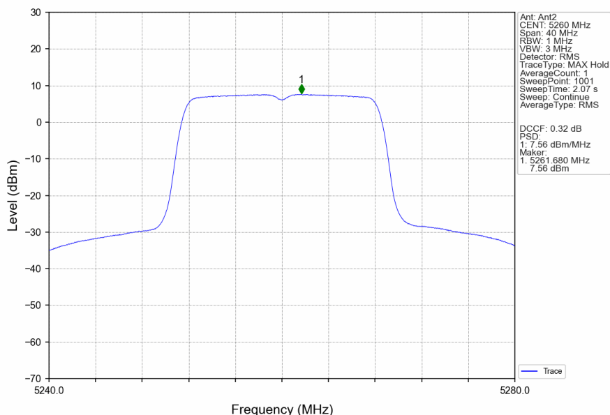
802.11a_LCH_5260MHz_Ant2_NTNV
