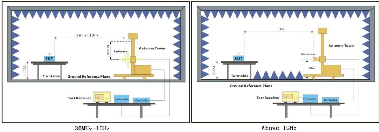
30MHz-1GHz
