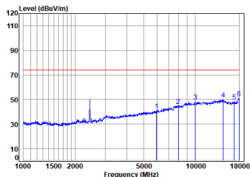
11ax_20M_TX_CH_06_Horizontal-Peak
