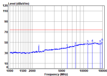
11ax_20M_TX_CH_11_Horizontal-Peak
