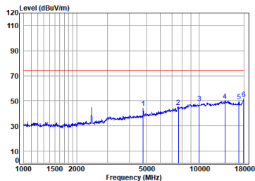
11ax_20M_TX_CH_06_Vertical-Peak
