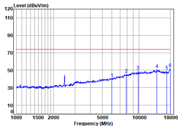
11ax_20M_TX_CH_11_Vertical-Peak
