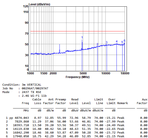
11b_TX_CH_06_Vertical-Peak
