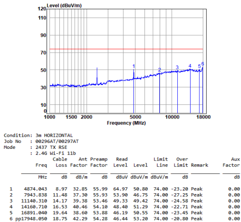
11b_TX_CH_06_Horizontal-Peak
