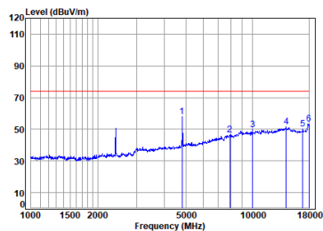
11b_TX_CH_01_Vertical-Peak
