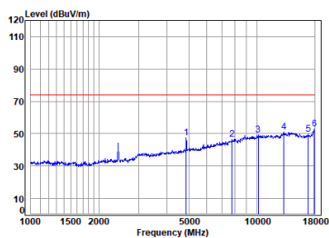
11n_20M_TX_CH_06_Horizontal-Peak
