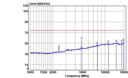
11g_TX_CH_01_Vertical-Peak
