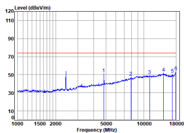
11b_TX_CH_01_Horizontal-Peak
