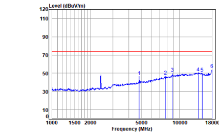
11g_TX_CH_01_Horizontal-Peak
