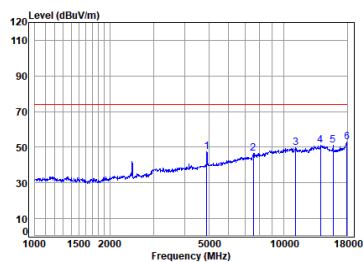
11g_TX_CH_11_Horizontal-Peak
