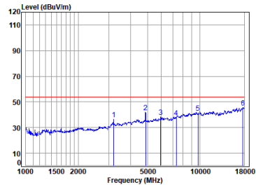
BLE_1M_TX_CH_19_Vertical-Avg
