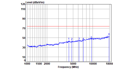
BLE_1M_TX_CH_00_Horizontal-Peak
