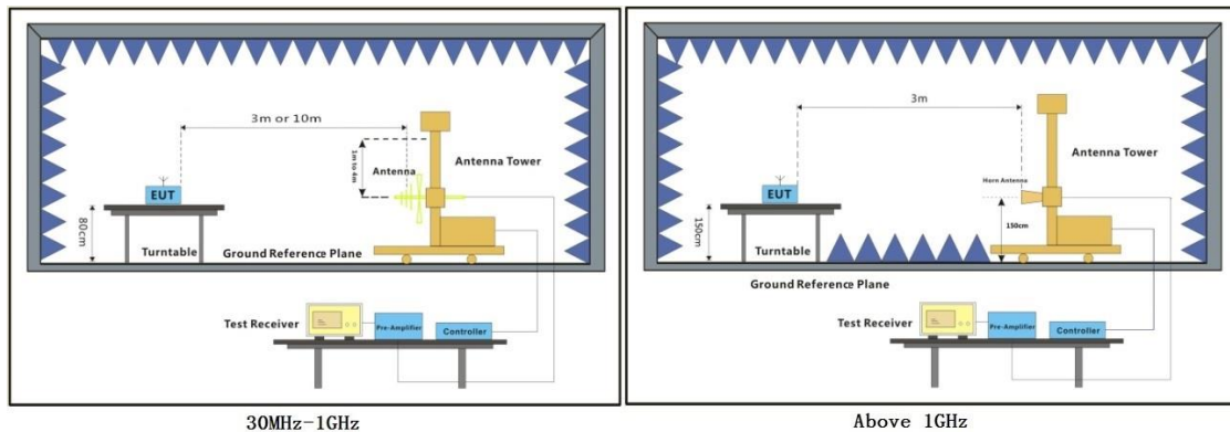
30MHz-1GHz
