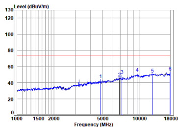
11g_TX_CH_01_Vertical-Peak
