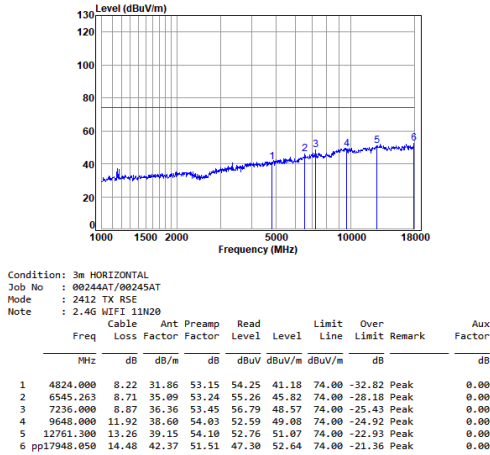
11n_20M_TX_CH_01_Horizontal-Peak
