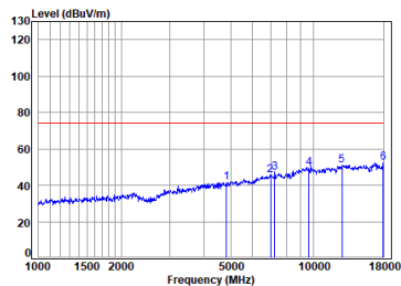
11g_TX_CH_01_Horizontal-Peak
