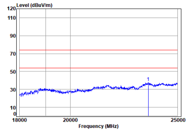
BLE_1M_TX_CH_00_Vertical-Peak
