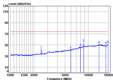
BLE_2M_TX_CH_39_Horizontal-Peak
