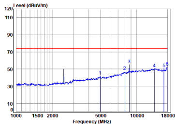
BLE_2M_TX_CH_39_Vertical-Peak
