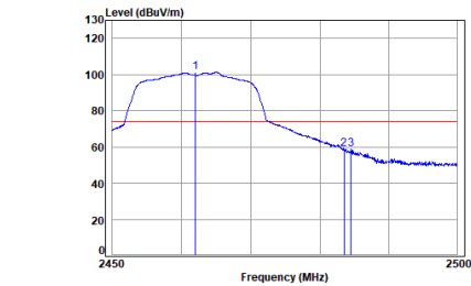
11n_HT(20M)_TX_CH_11_Vertical-Peak
