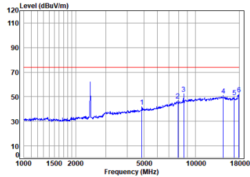
11n_20M_TX_CH_06_Horizontal-Peak
