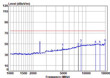
11b_TX_CH_11_Horizontal-Peak
