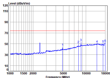
11b_TX_CH_11_Vertical-Peak
