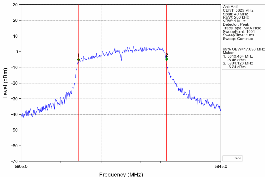
802.11ac(VHT20)_HCH_5825MHz_Ant1_NTNV
