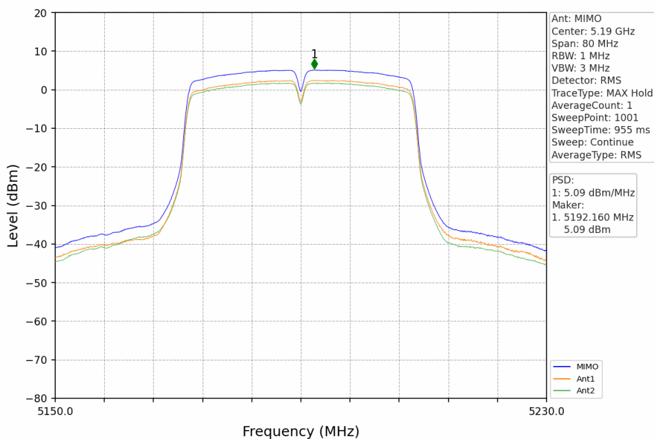
802.11ac(VHT40)_LCH_5190MHz_MIMO_NTNV
