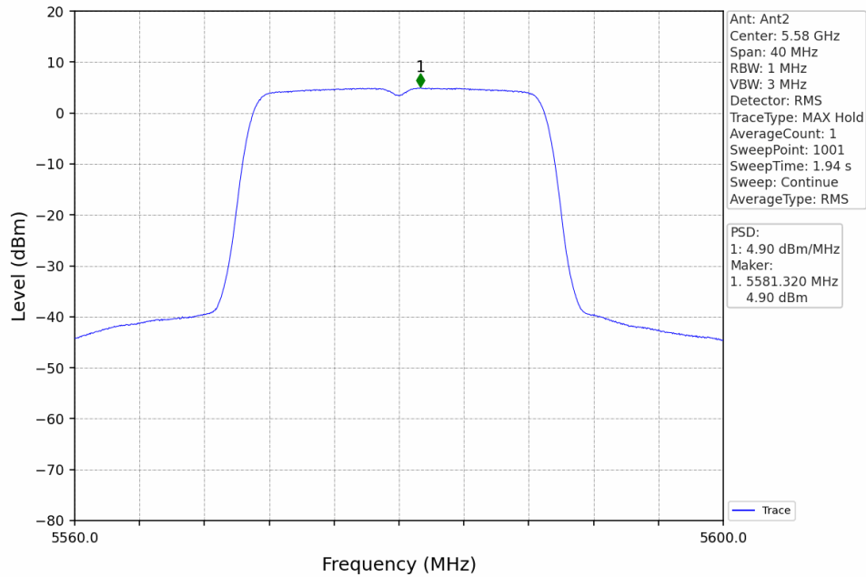
802.11ac(VHT20)_MCH_5580MHz_MIMO_NTNV
