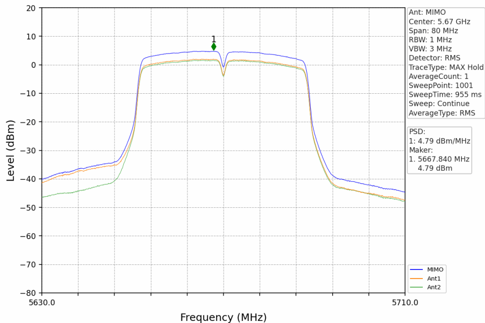
802.11ac(VHT40)_HCH_5670MHz_MIMO_NTNV
