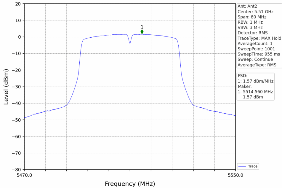
802.11ac(VHT40)_LCH_5510MHz_MIMO_NTNV
