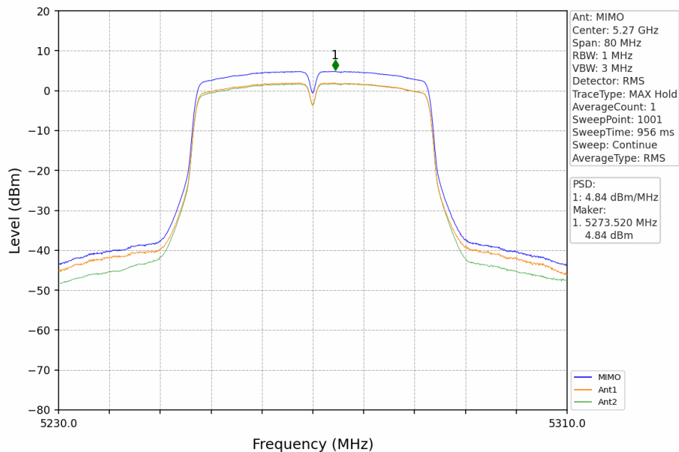
802.11ac(VHT40)_LCH_5270MHz_MIMO_NTNV
