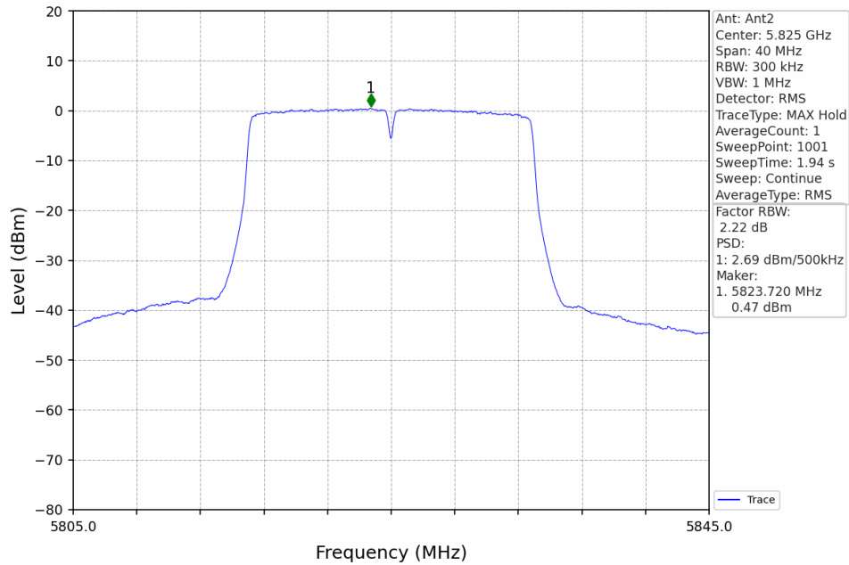
802.11ac(VHT20)_HCH_5825MHz_MIMO_NTNV
