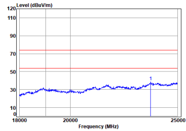
BLE_1M_TX_CH_19_Vertical-Peak
