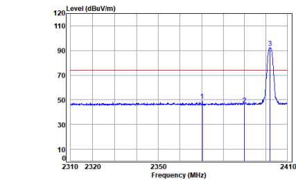
BLE_1M_TX_CH_00_Vertical-Peak
