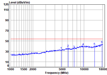
BLE_1M_TX_CH_19_Horizontal-Avg
