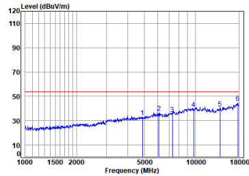
BLE_1M_TX_CH_19_Vertical-Avg
