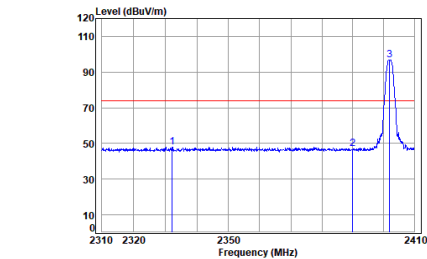
BLE_1M_TX_CH_00_Horizontal-Peak
