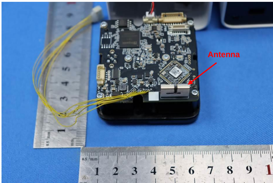
Version B (Ying Jia Chuang Antenna)
