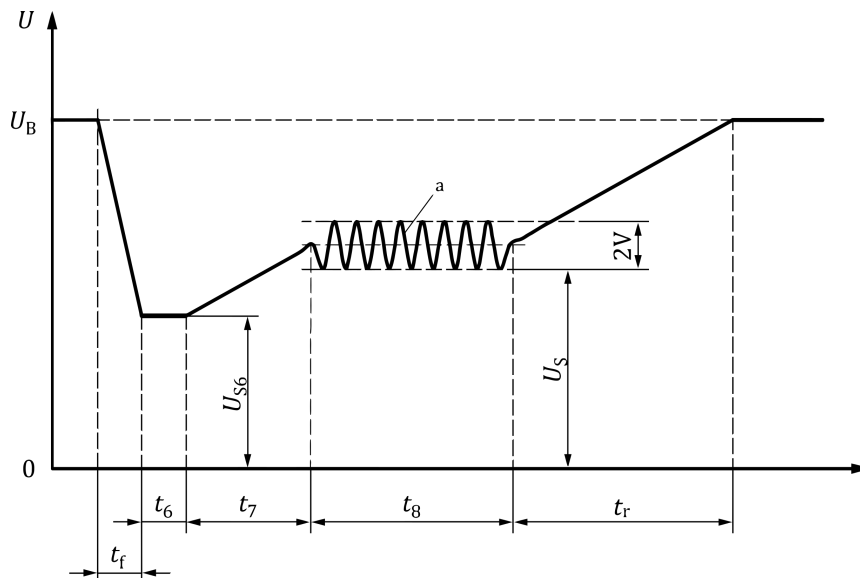
Figure 4: ISO 16750-2, Figure 7 – Starting profile
