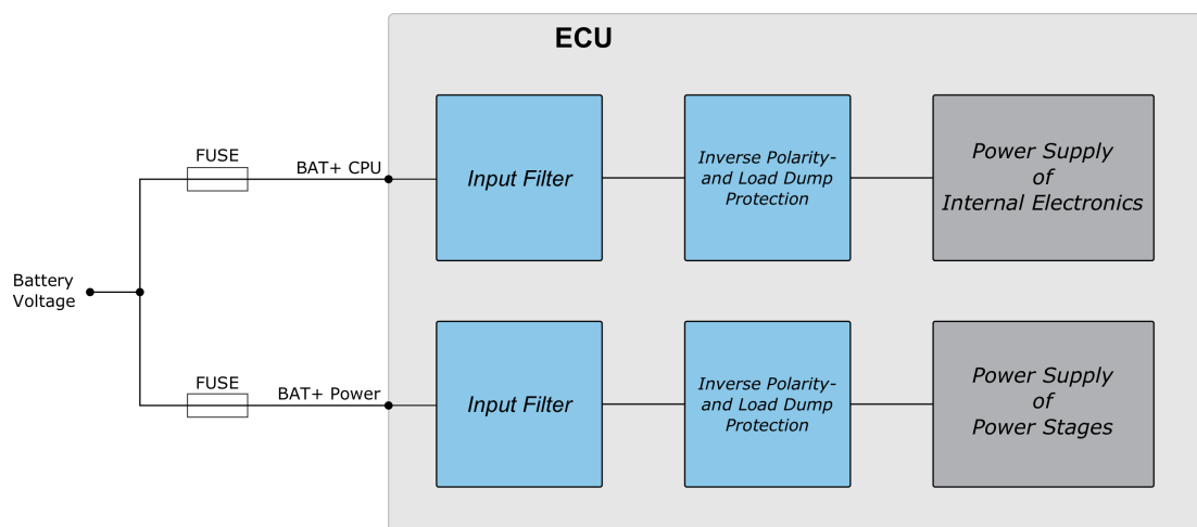
Figure 2: Battery supply – Fuse
