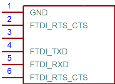
Figure 25: Pinning schematic for the USB-FDTI connector
