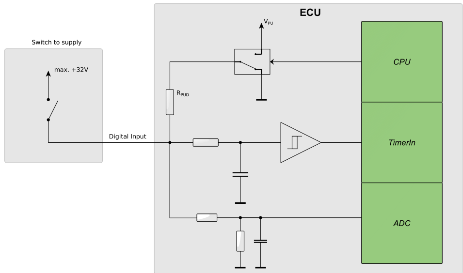
Figure 15: Digital input for switch connected to (battery) supply voltage
