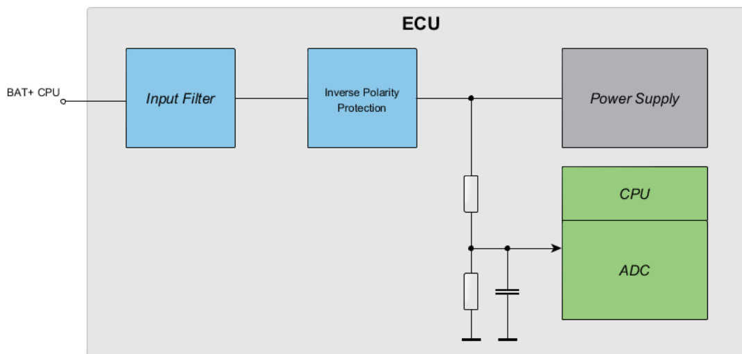
Figure 3: Supply pin for the internal ECU logic
