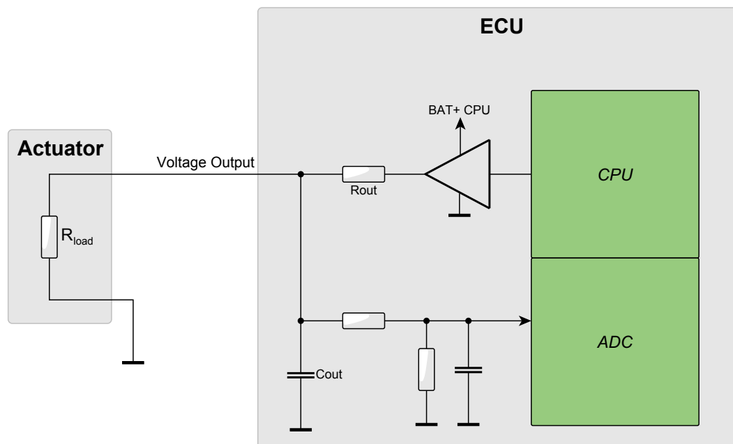
Figure 21: Output stage in V_{OUT} mode
