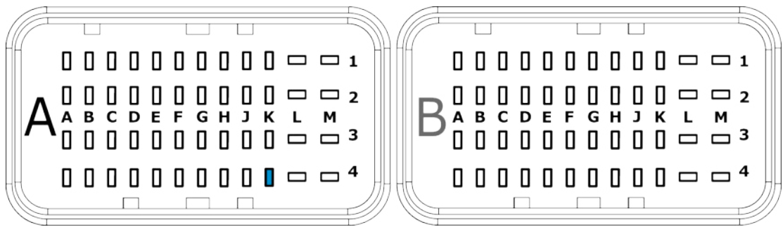
Figure 51: LIN pinout
