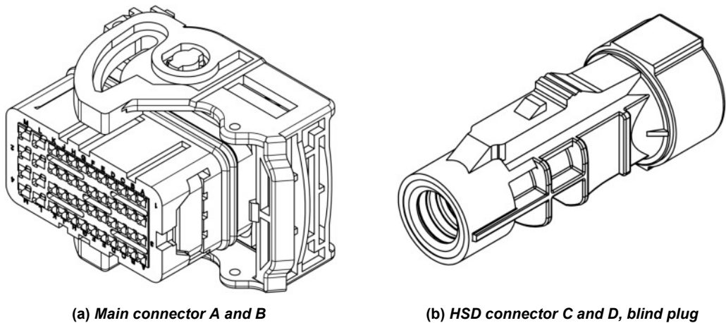
Figure 5: Plug housings
