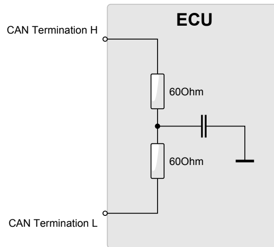
Figure 56: CAN termination
