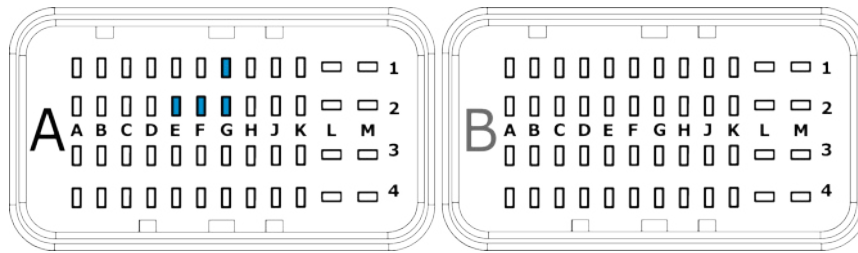
Figure 41: PWM LS 4A+CM pinout
