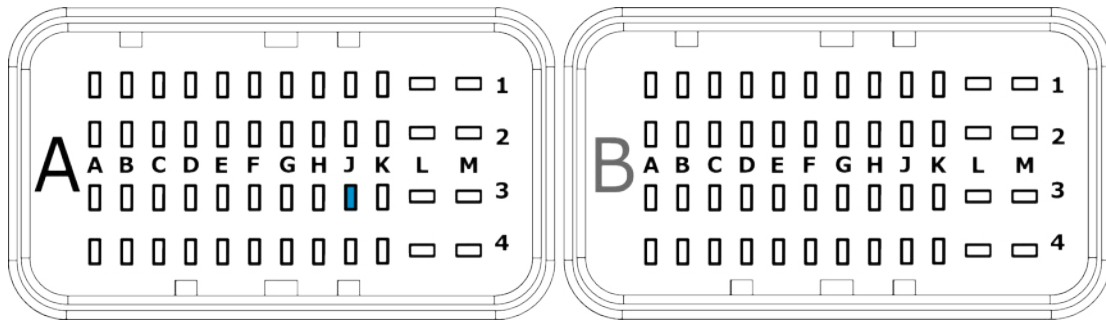
Figure 15: T15 pinout
