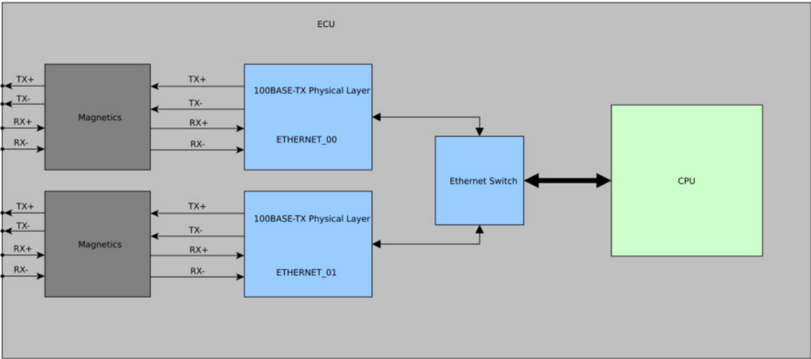
Figure 59: Ethernet interface
