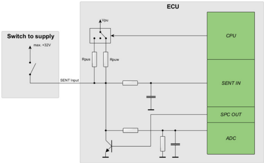
Figure 33: Digital input for switch connected to (battery) supply voltage
