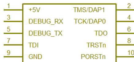
Figure 66: Pinning schematic for the ECU interface
