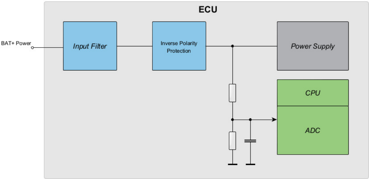
Figure 11: Supply pin for the internal ECU logic for BAT+ Power
