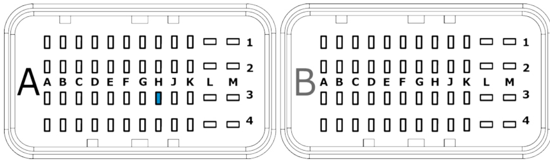
Figure 16: Wake-up pinout
