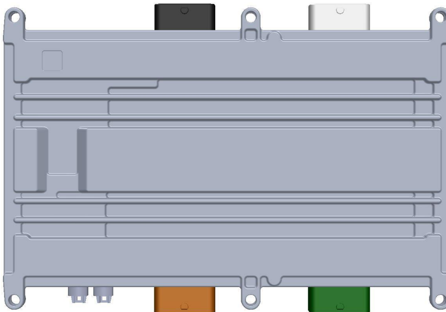
Figure 4: Bottom view
