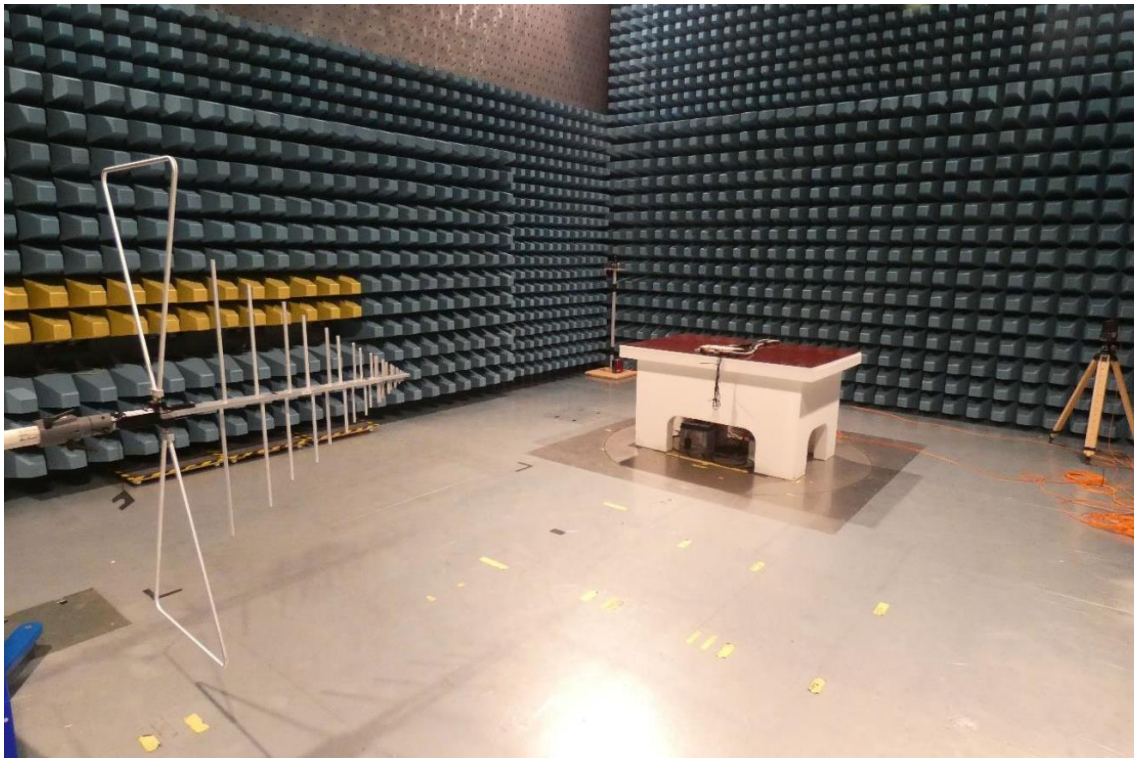
Figure 2: Radiated Emission 30 MHz – 1000 MHz
