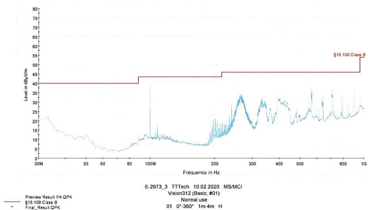
Chart 1: Radiated emissions, 30 - 1000 MHz, horizontal
