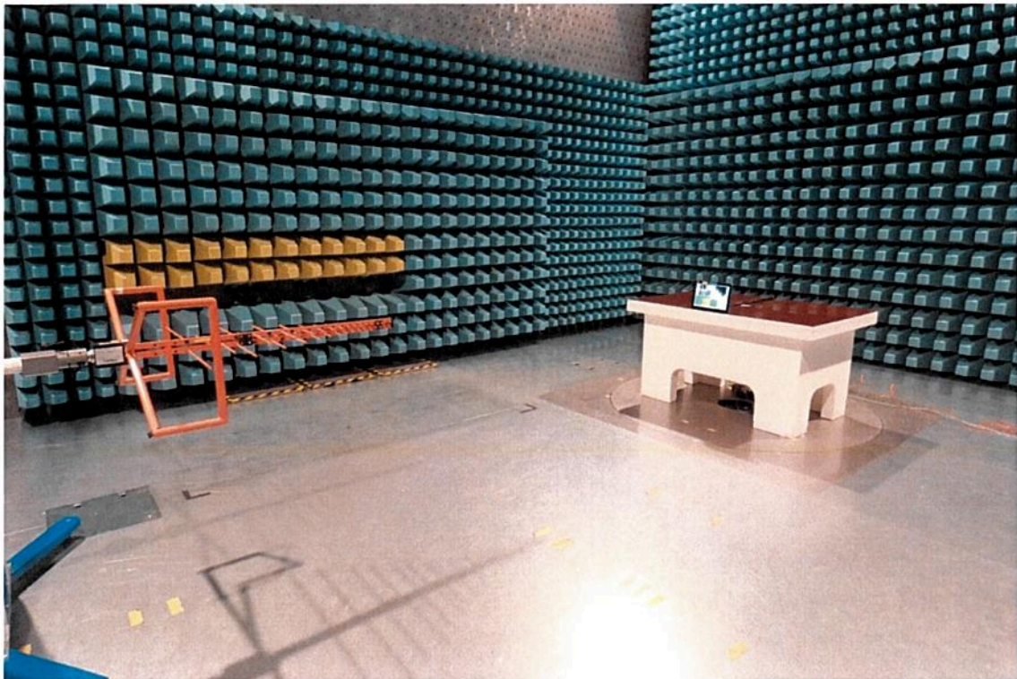
Photo 3: Setup in the Semi anechoic chamber (SAC3) radiated emissions measurement (30 MHz – 1000 MHz)
