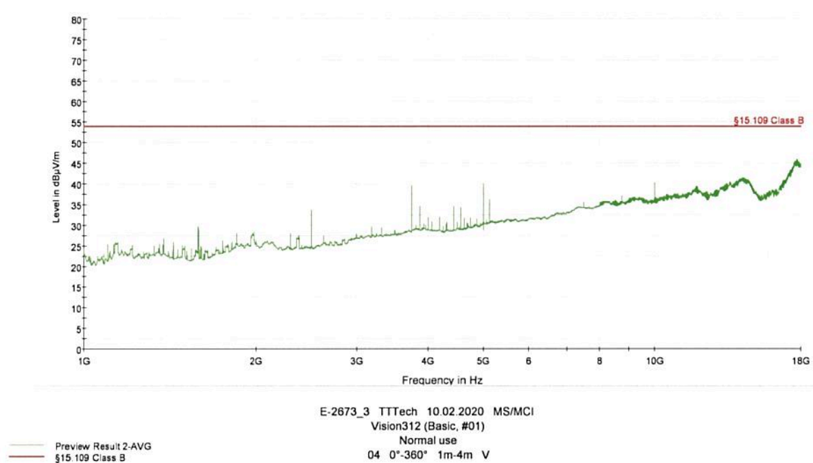
Chart 4: Radiated emissions, 1000 - 18000 MHz, vertical
