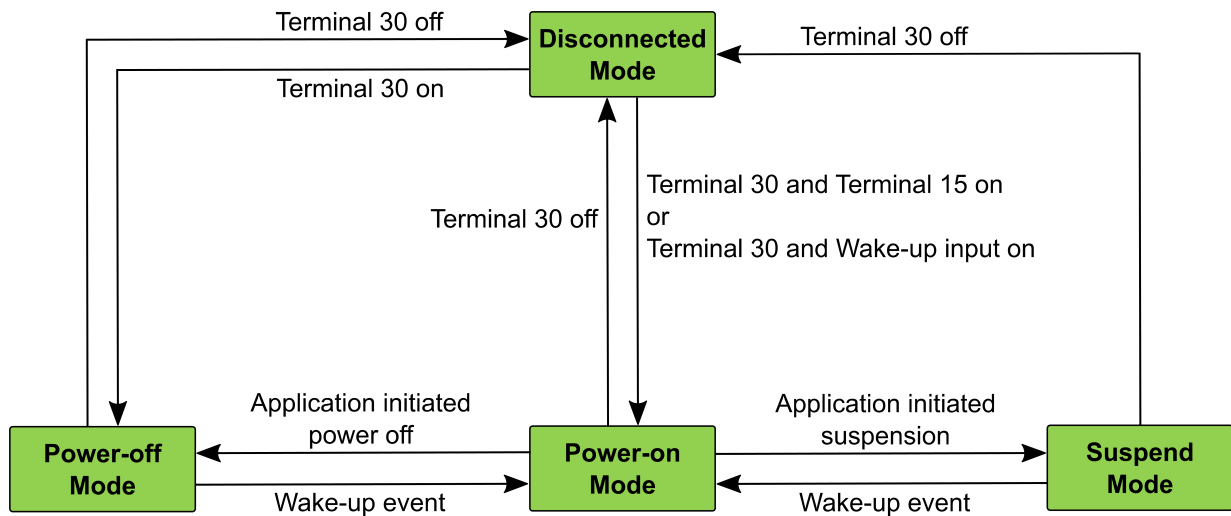
Figure 10: Power modes
