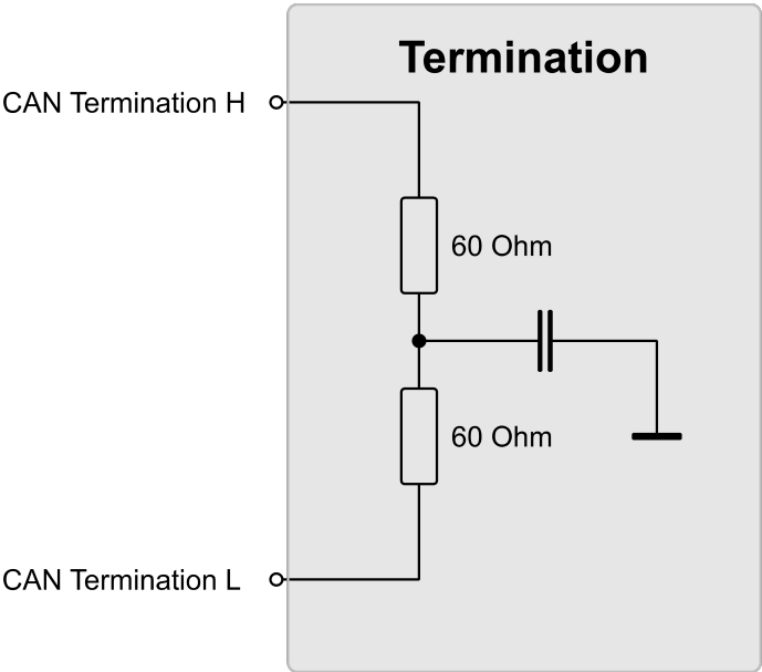
Figure 9: CAN termination
