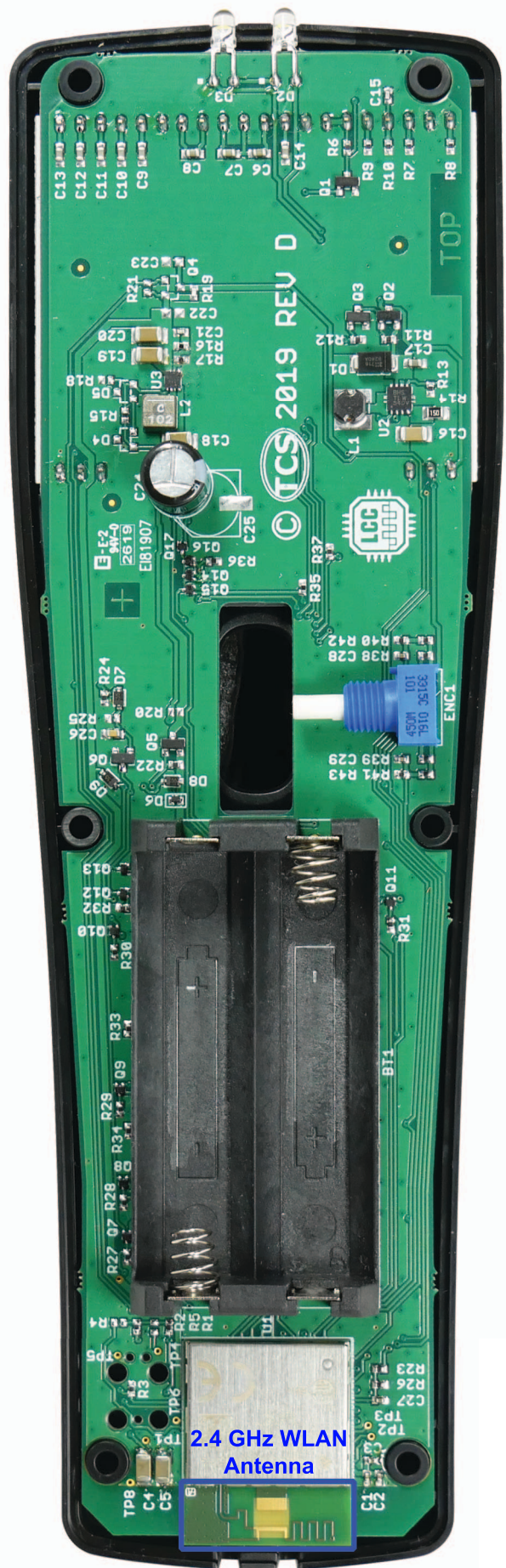
PCB Viewed From Back (back of case removed)
