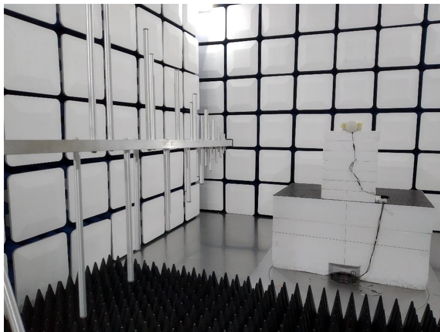
960MHz-1GHz
