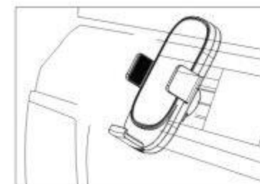
3.Insert the clip into the blade of the air vent
