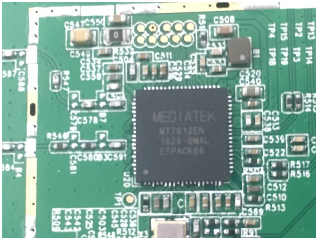
5G Chip
