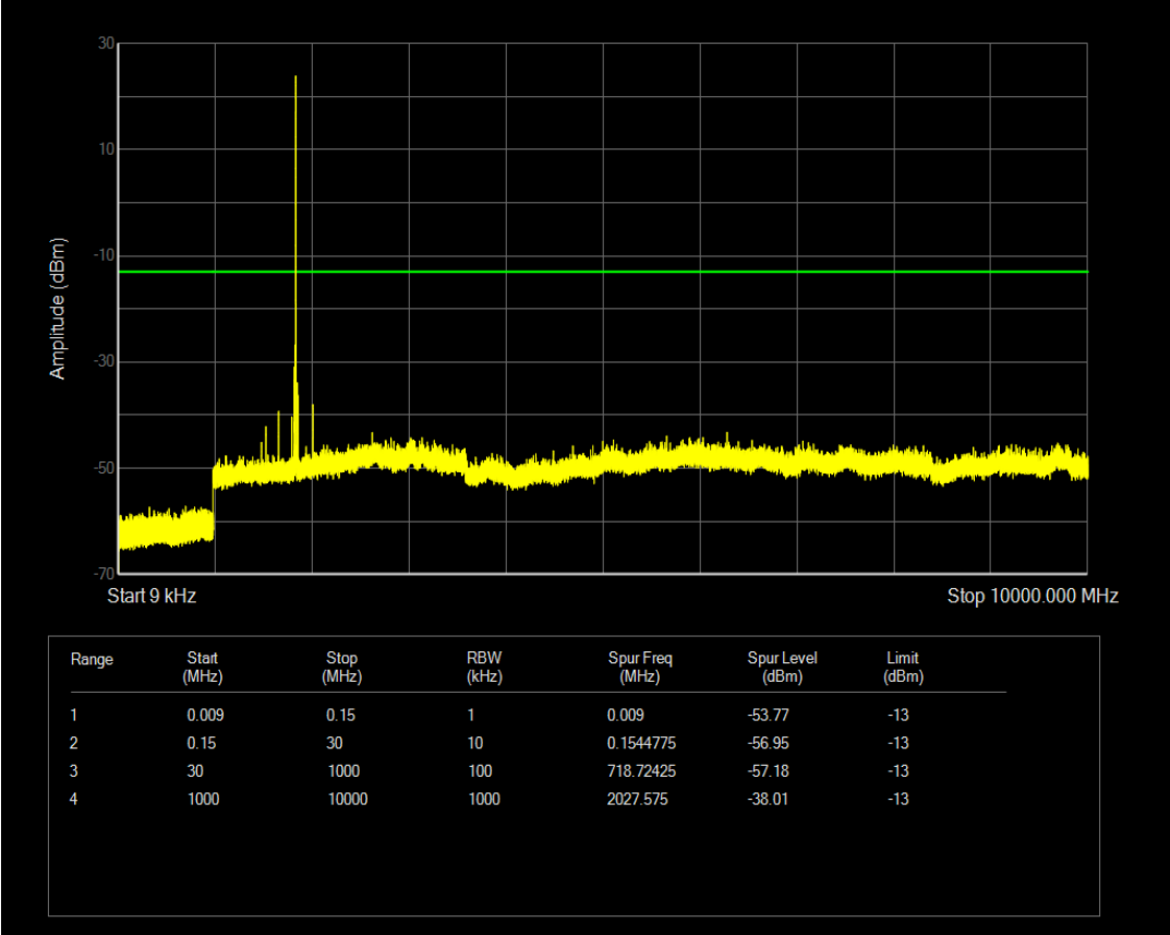
Band2 QAM16 BW=10MHz Channel=18650 RB Size=6 Position=#0 NB Index=0
