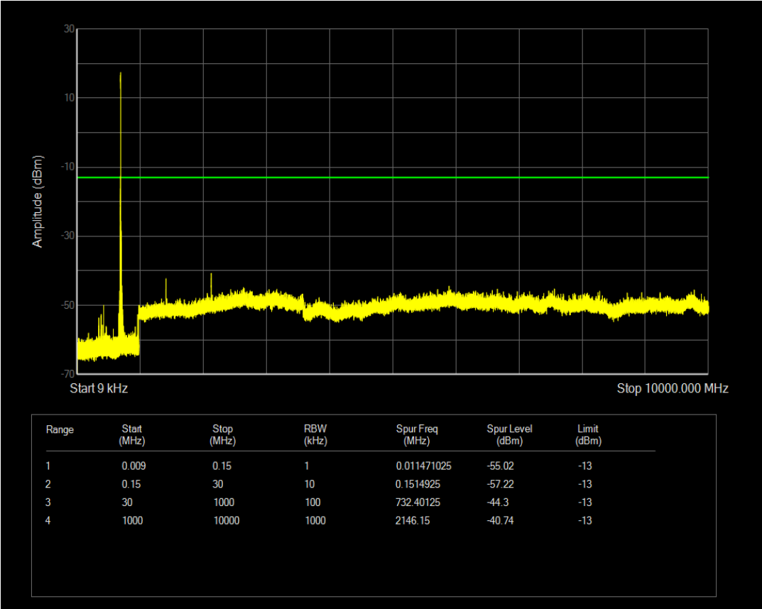
Band12 QAM16 BW=1.4MHz Channel=23173 RB Size=1 Position=#0 NB Index=0
