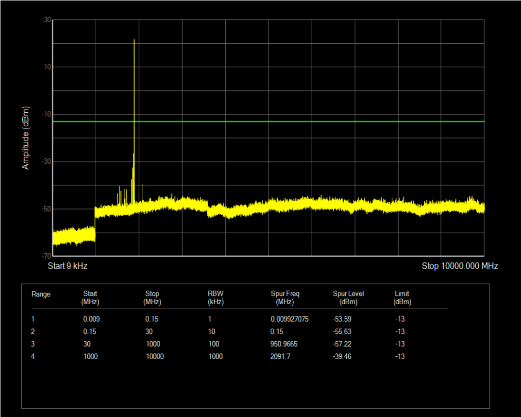
Band2 QAM16 BW=1.4MHz Channel=19193 RB Size=1 Position=#0 NB Index=0
