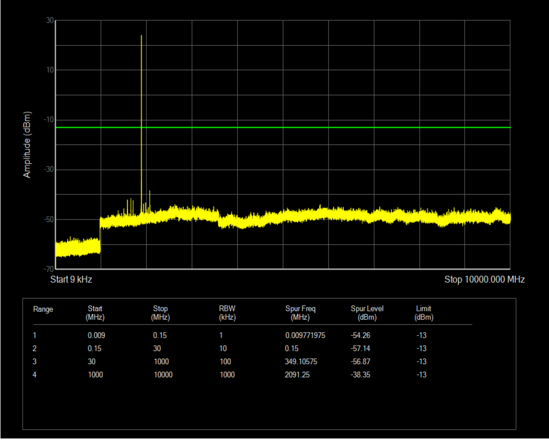
Band2 QAM16 BW=1.4MHz Channel=19193 RB Size=6 Position=#0 NB Index=0
