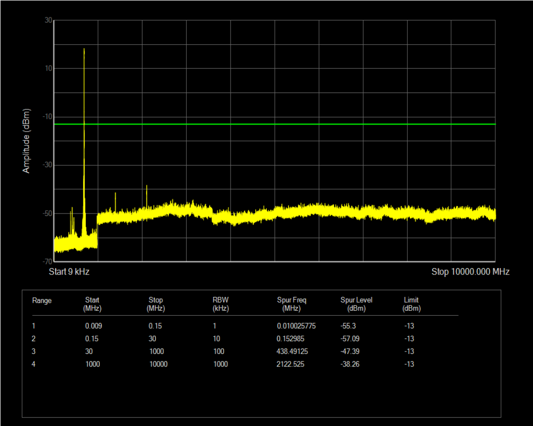
Band12 QAM16 BW=10MHz Channel=23130 RB Size=1 Position=#0 NB Index=0
