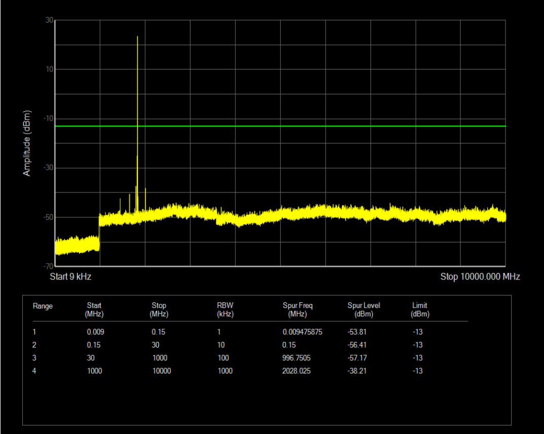
Band2 QAM16 BW=15MHz Channel=18675 RB Size=6 Position=#0 NB Index=0
