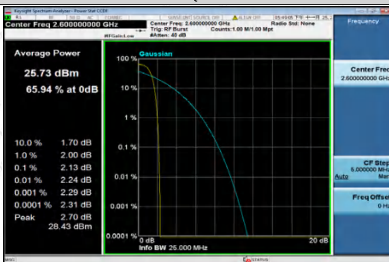
Band41-10MHz-QPSK-40690-50RB#0
