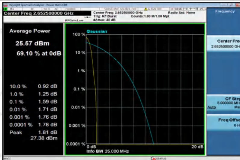
Band41-5MHz-QPSK-41215-25RB#0
