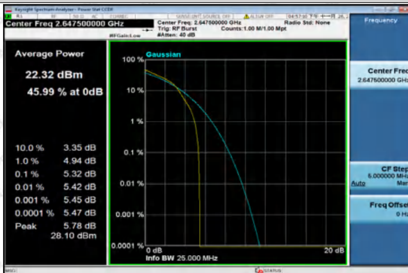
Band41-15MHz-16QAM-41165-5RB#0
