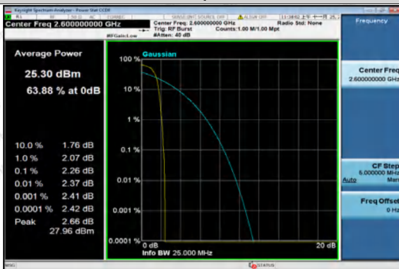
Band41-5MHz-16QAM-40690-25RB#0
