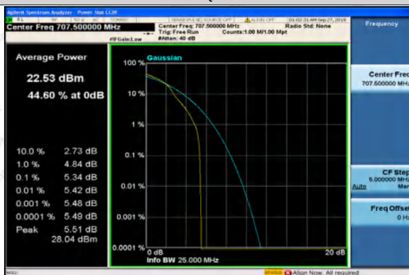
Band12-3MHz-16QAM-23095-15RB#0
