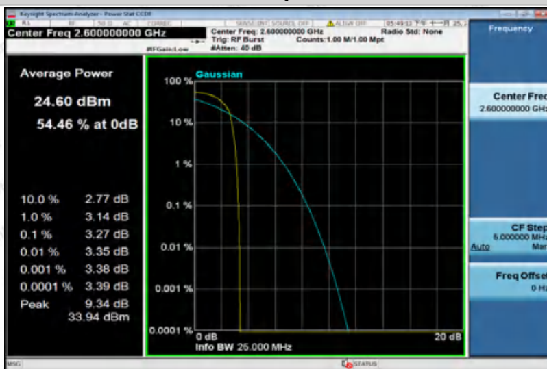
Band41-10MHz-16QAM-40690-50RB#0
