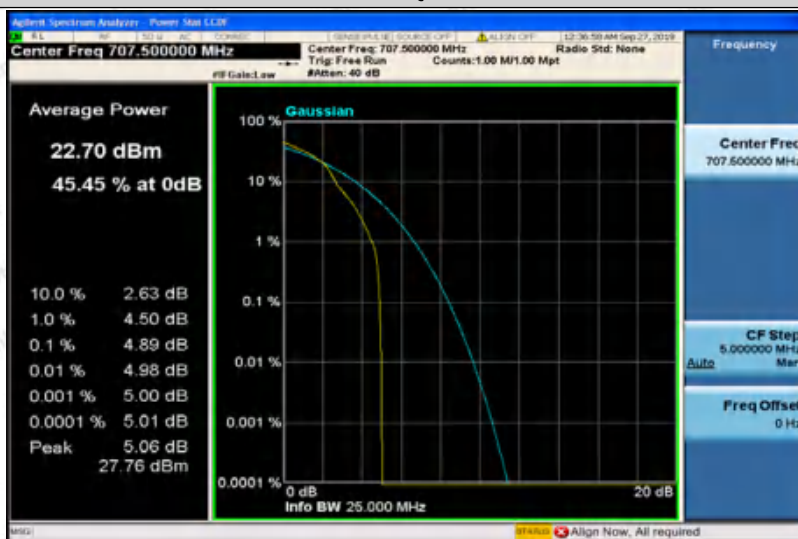
Band12-1.4MHz-16QAM-23095-6RB#0
