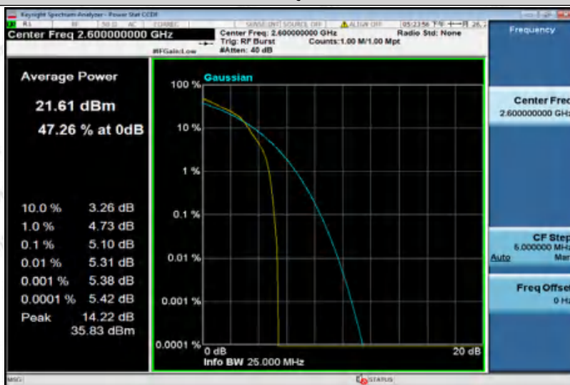
Band41-20MHz-16QAM-40690-100RB#0
