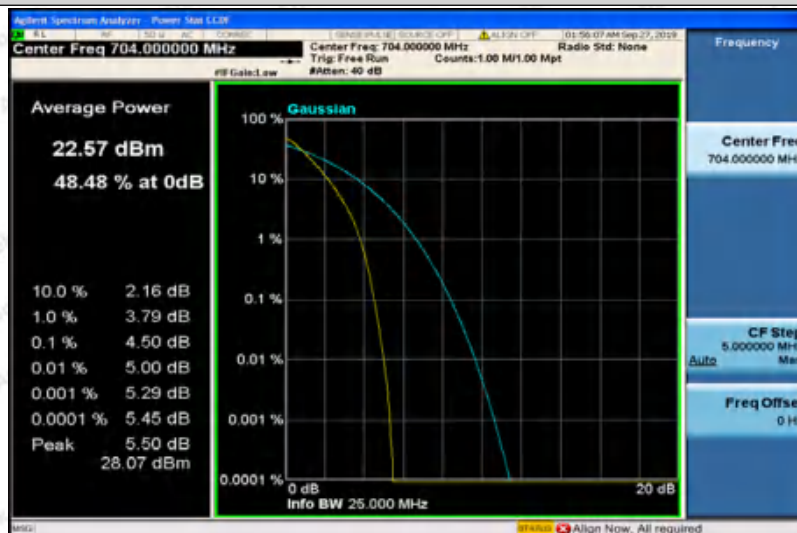
Band12-10MHz-QPSK-23095-1RB#0
