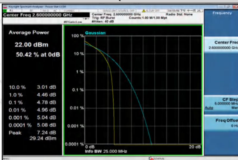
Band41-15MHz-QPSK-40690-75RB#0
