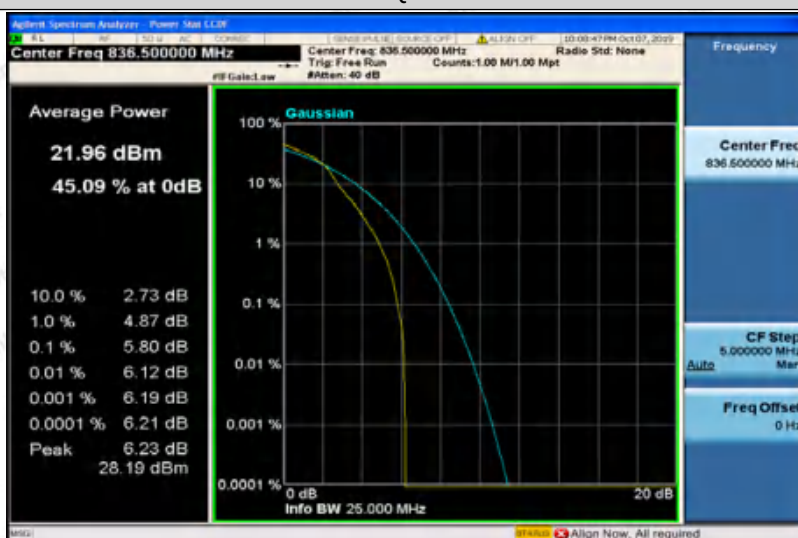
Band5-3MHz-16QAM-20525-15RB#0
