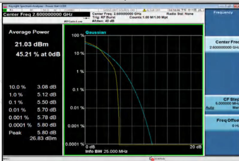
Band41-15MHz-16QAM-40690-75RB#0
