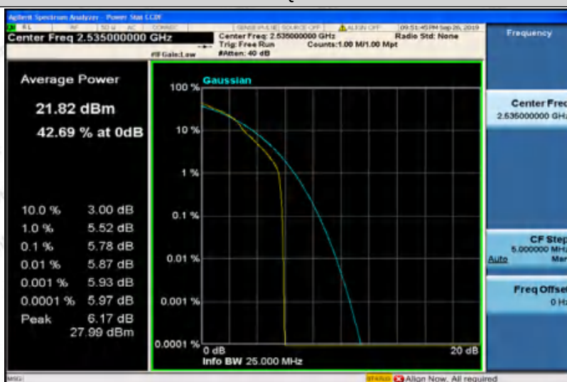
Band7-20MHz-16QAM-21100-100RB#0
