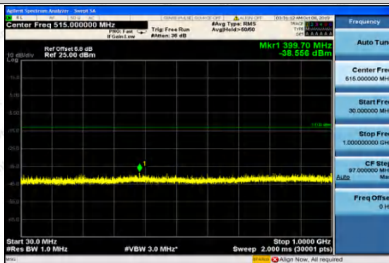
GPRS1900-512-30~1000
