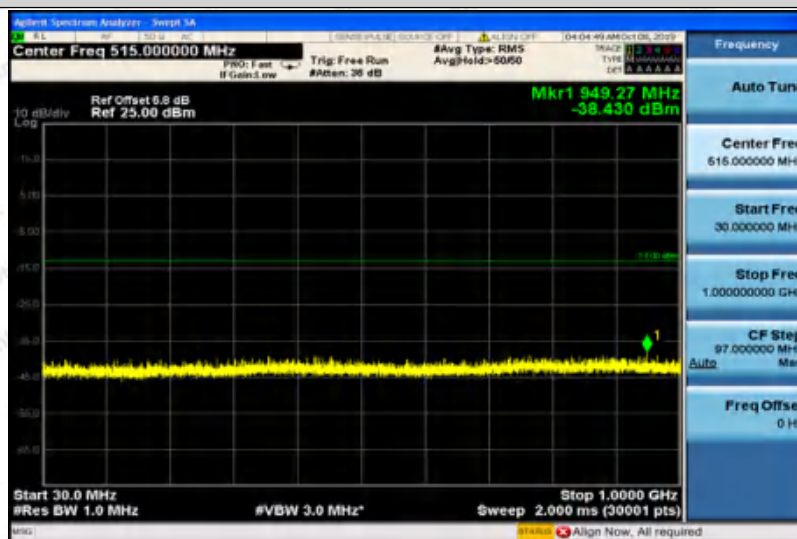
EGPRS1900-512-30~1000
