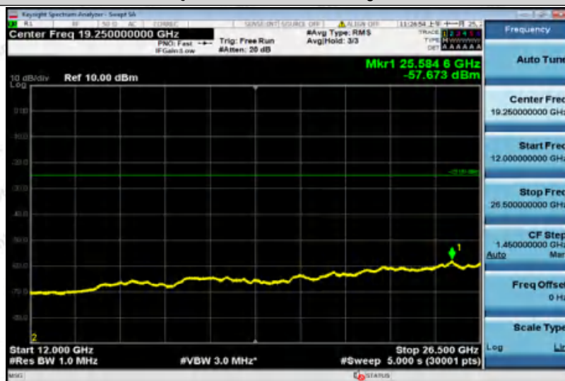
Band41-5MHz-16QAM-40690-1RB#0-Range1:30~1000MHz
