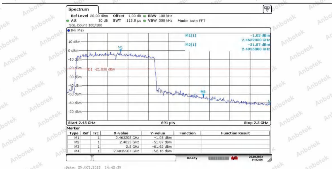
11AX20SISO_Ant2_High_2462
