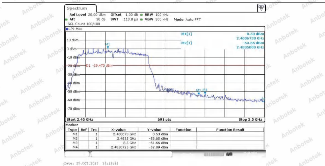
11N20SISO_Ant2_High_2462
