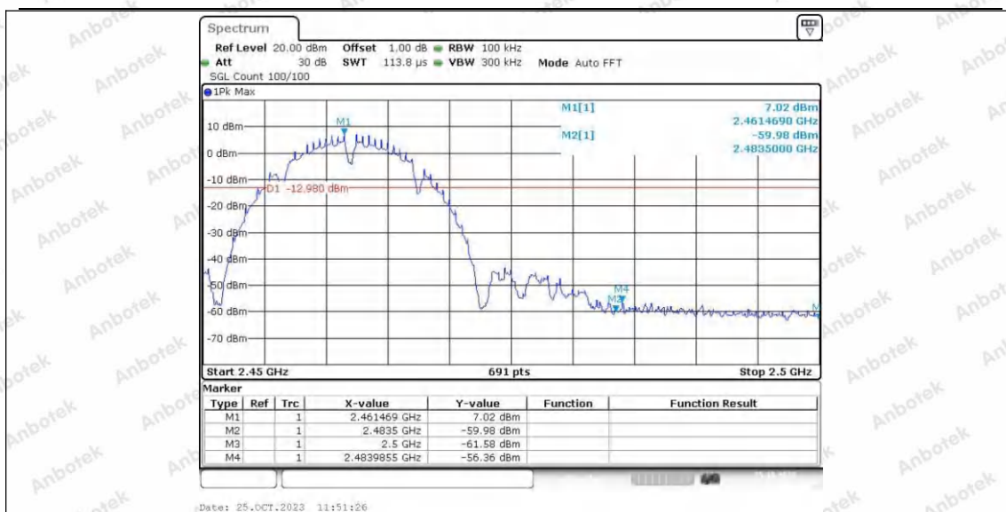
11B_Ant2_High_2462
