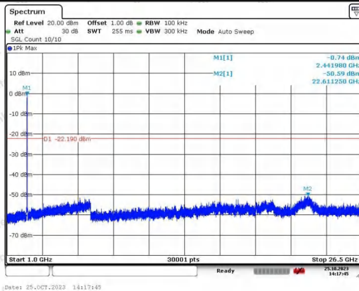
11N20SISO_Ant2_2437_0~Reference
