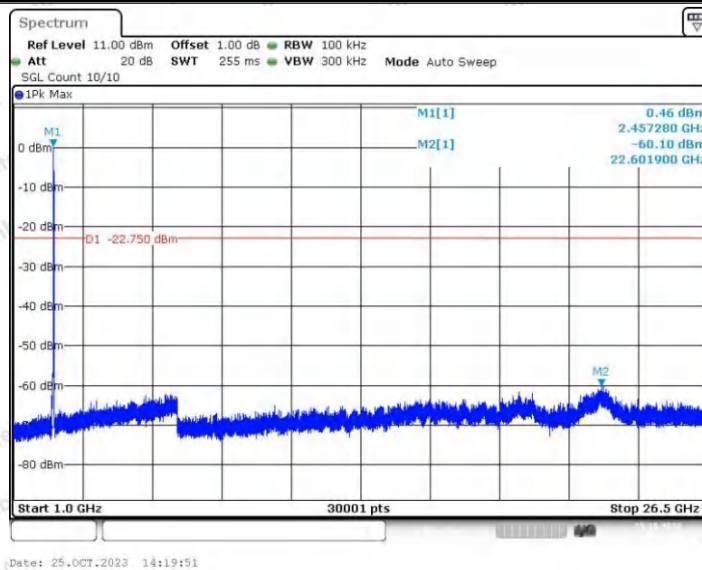
11N20SISO_Ant2_2462_0~Reference
