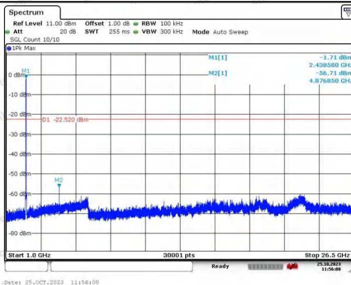
11G_Ant2_2437_0~Reference
