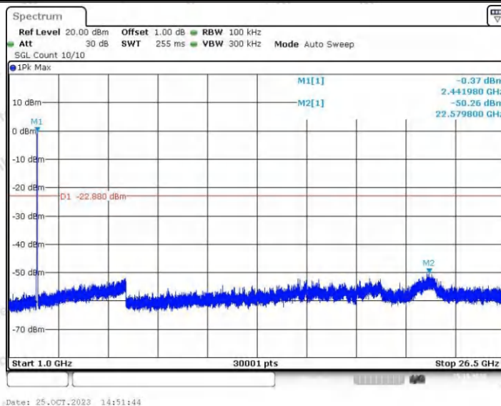
11AX40SISO_Ant2_2437_0~Reference
