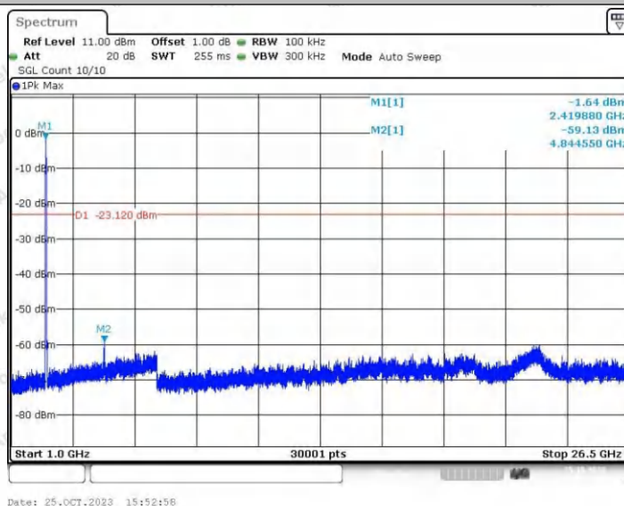
11AX40SISO_Ant1_2437_0~Reference
