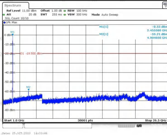
11N40SISO_Ant2_2452_0~Reference
