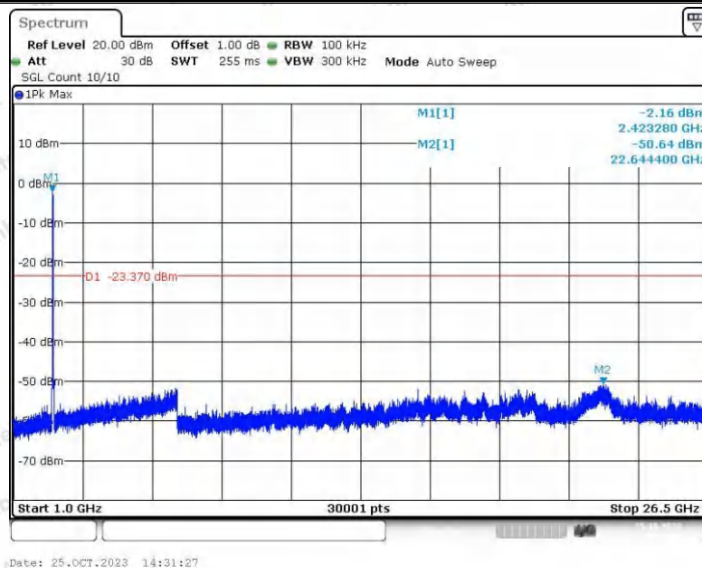
11N40SISO_Ant2_2437_0~Reference
