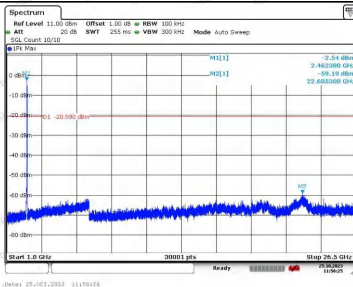
11G_Ant2_2462_0~Reference
