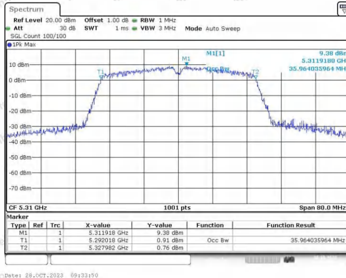
11AC40SISO_Ant2_5310
