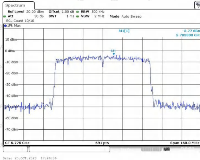
11AC80SISO_Ant2_5775
