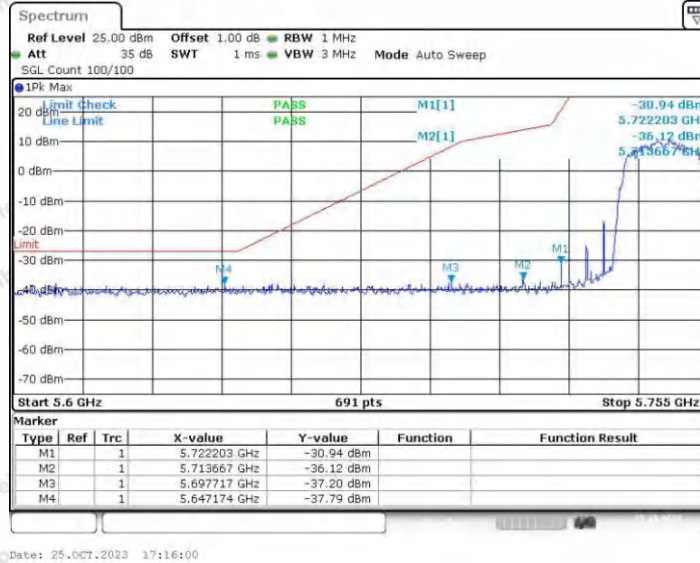
11AC20SISO_Ant2_Low_5745
