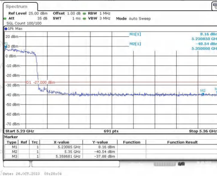
11AX40SISO_Ant2_High_5230
