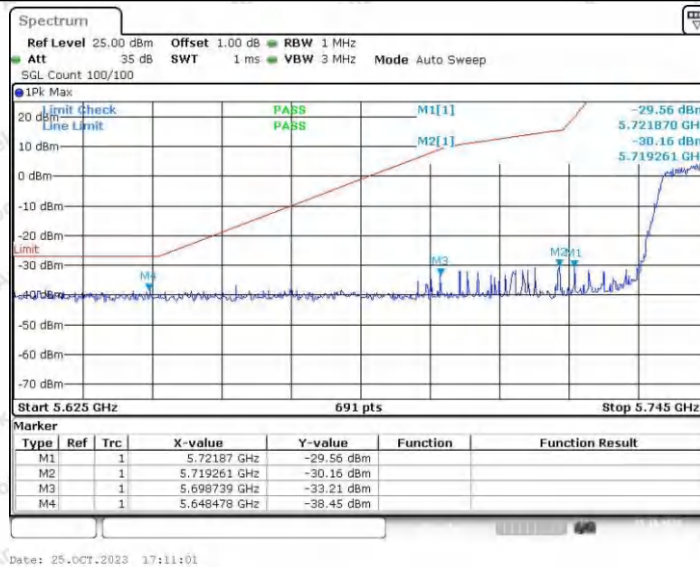
11N40SISO_Ant2_Low_5755
