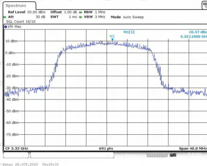
11AC20SISO_Ant2_5320
