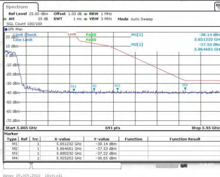
11AC40SISO_Ant2_High_5795
