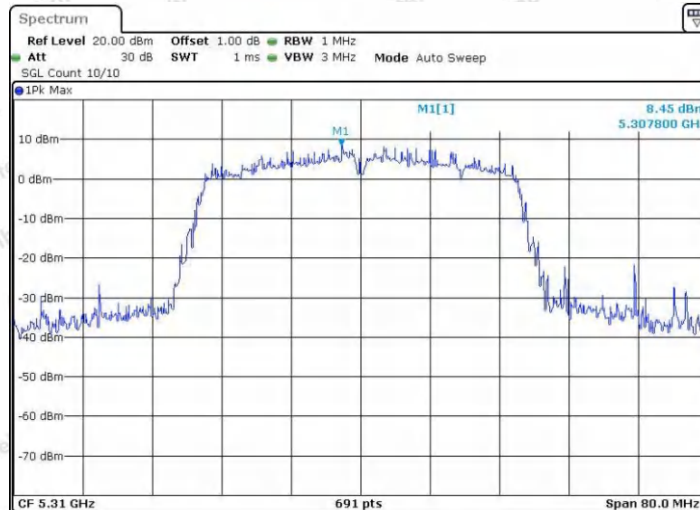
11N40SISO_Ant1_5310
