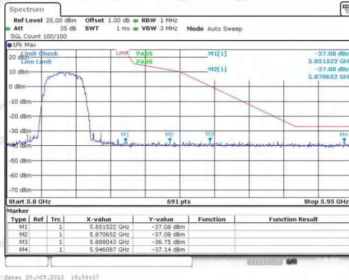
11A_Ant2_High_5825
