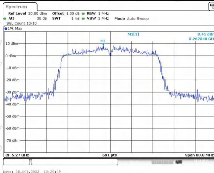
11AC40SISO_Ant2_5270
