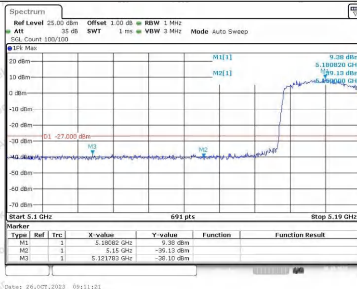
11AX20SISO_Ant2_Low_5180
