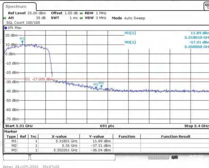
11AX20SISO_Ant1_High_5320
