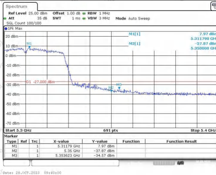
11AC40SISO_Ant2_High_5310
