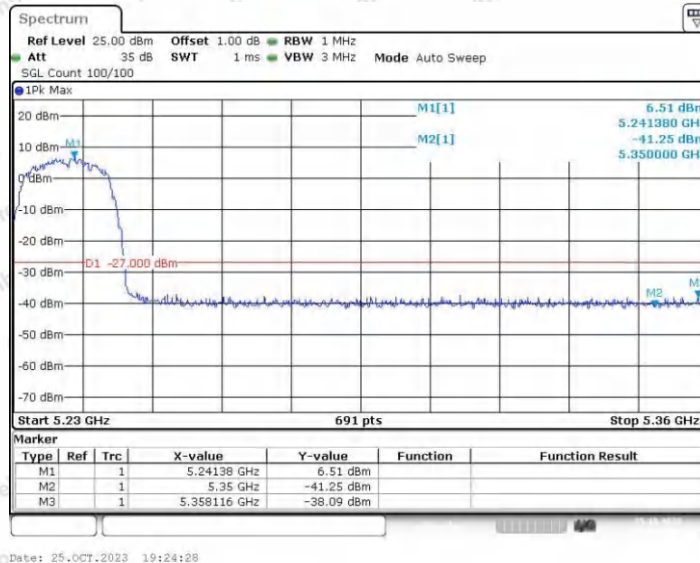
11A_Ant2_High_5240
