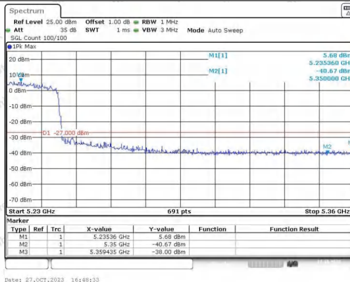
11AX40SISO_Ant2_High_5230
