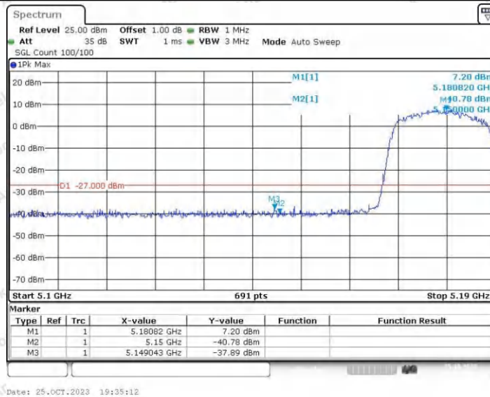
11N20SISO_Ant2_Low_5180
