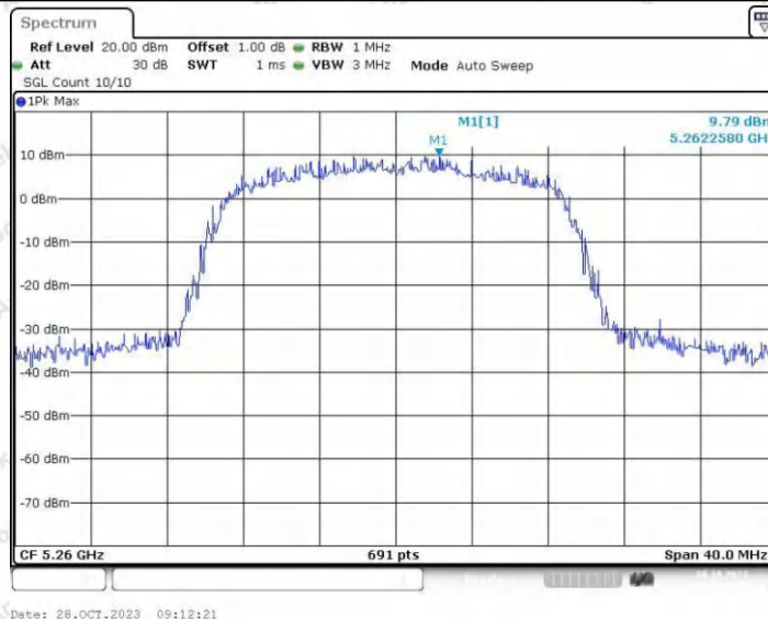
11N20SISO_Ant2_5260
