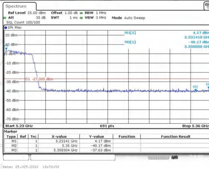
11N40SISO_Ant2_High_5230
