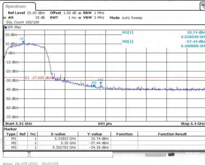
11N20SISO_Ant1_High_5320
