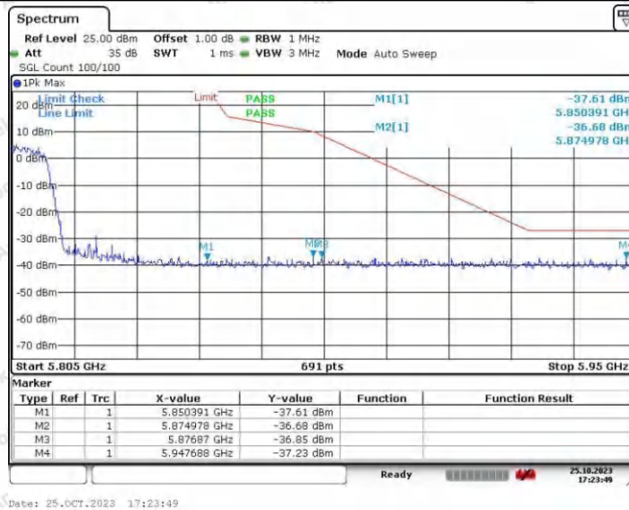
11AC40SISO_Ant2_High_5795
