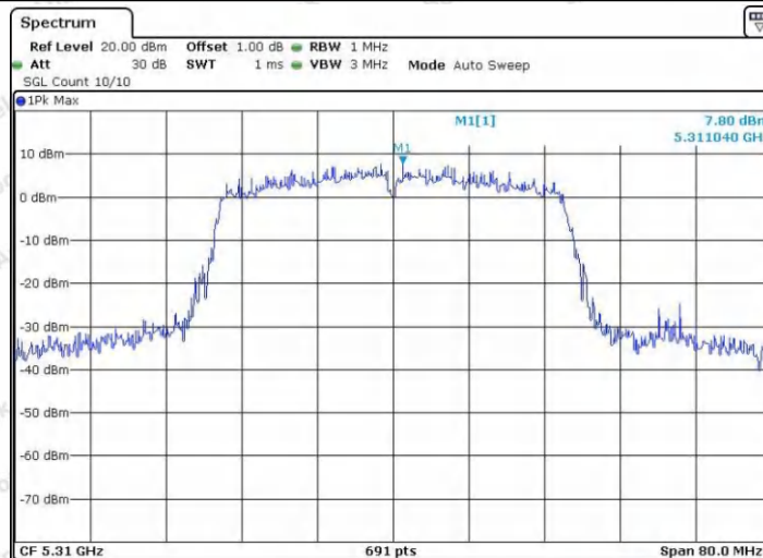
11N40SISO_Ant2_5310
