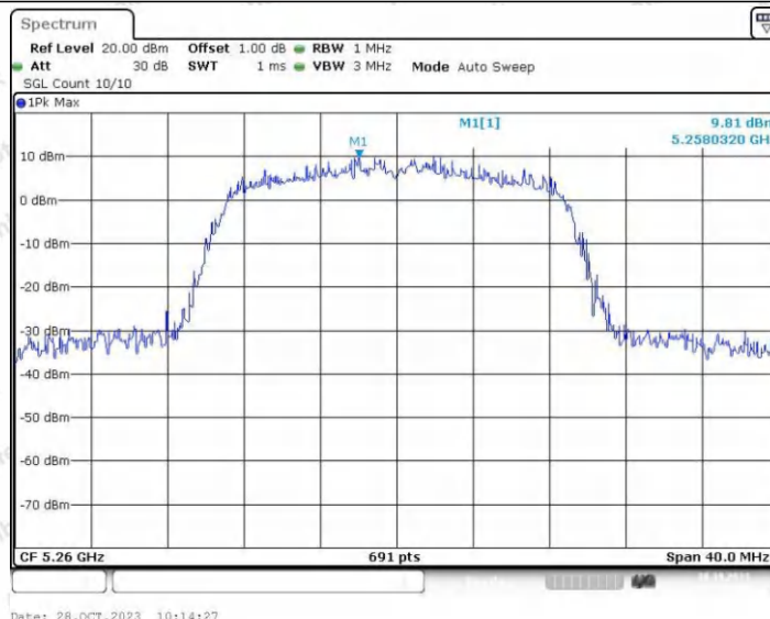
11AC20SISO_Ant2_5260
