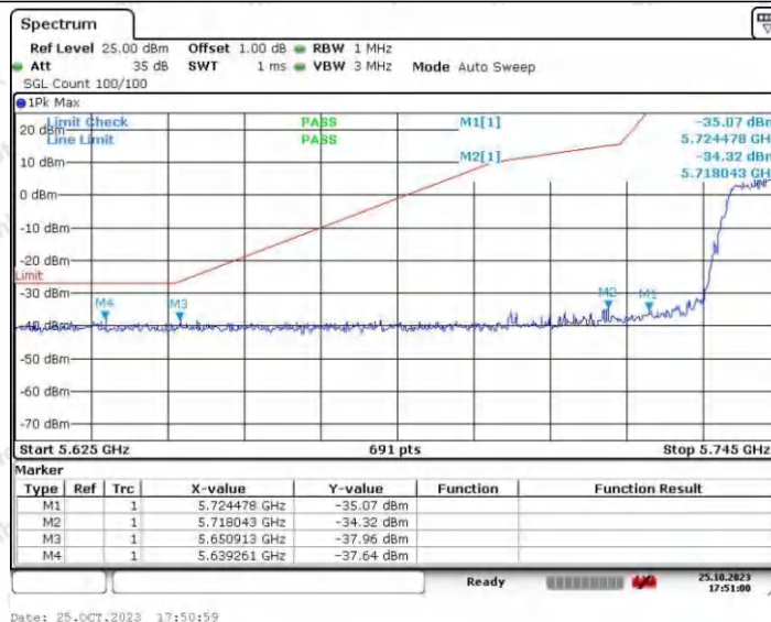
11N40SISO_Ant2_Low_5755
