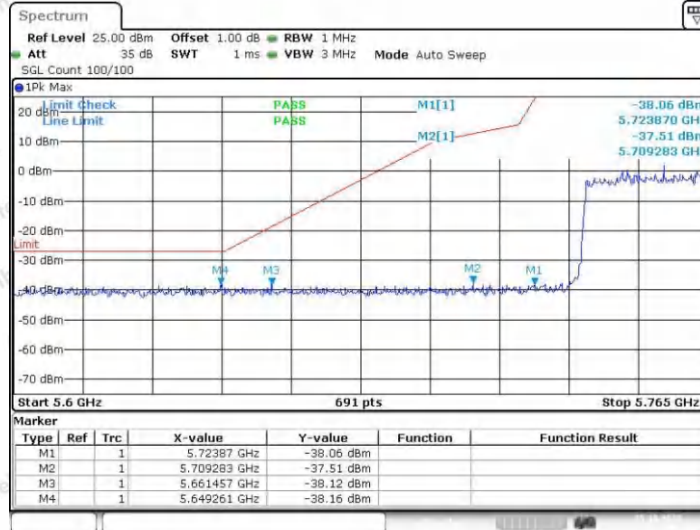
11AX80SISO_Ant1_High_5775
