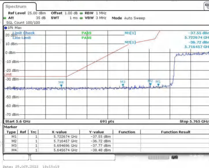
11AX80SISO_Ant2_Low_5775
