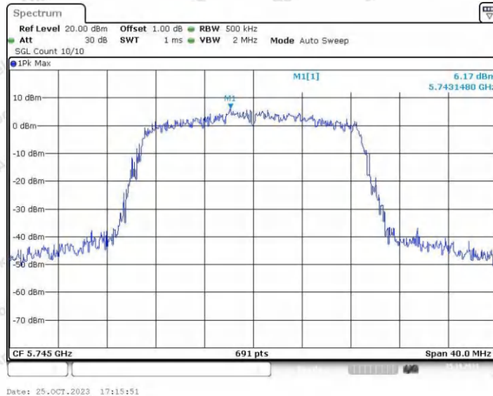
11AC20SISO_Ant2_5745
