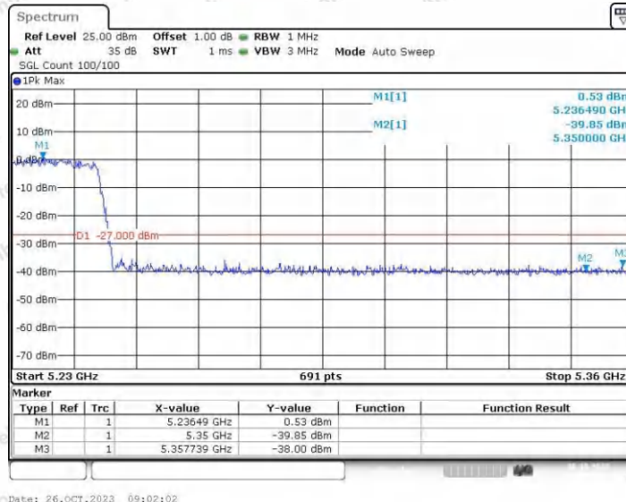
11AC80SISO_Ant2_High_5210
