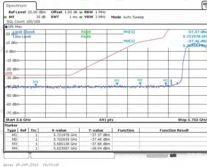
11A_Ant2_Low_5745
