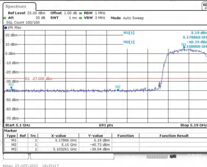
11N20SISO_Ant2_Low_5180
