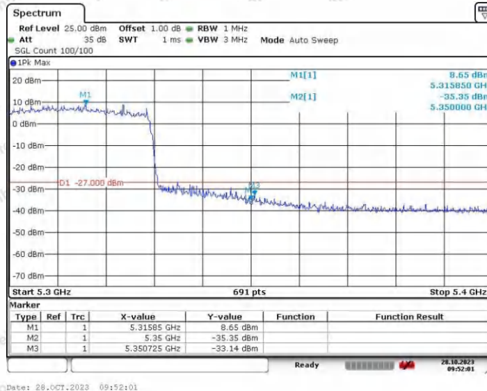
11AX40SISO_Ant2_High_5310
