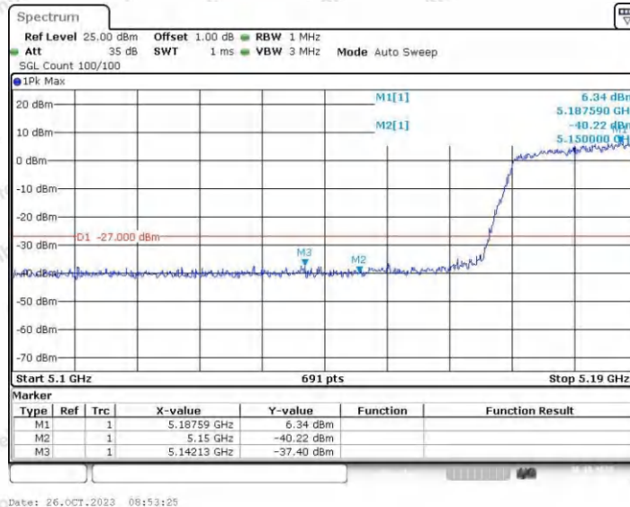
11AC40SISO_Ant2_Low_5190
