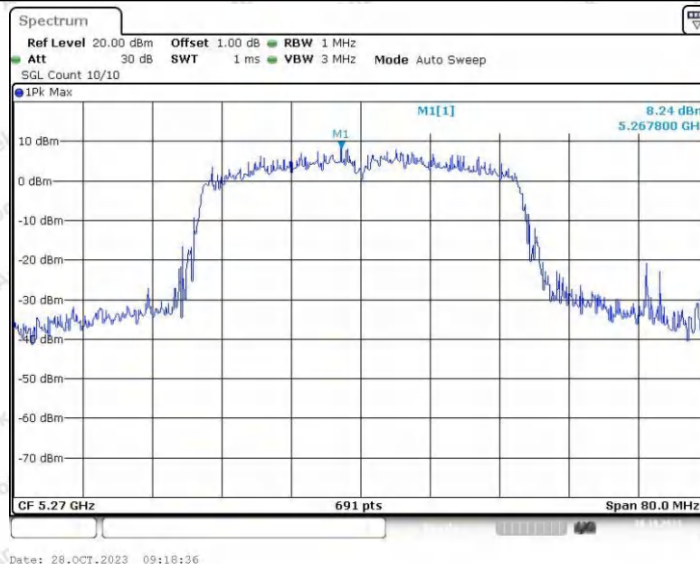
11N40SISO_Ant2_5270
