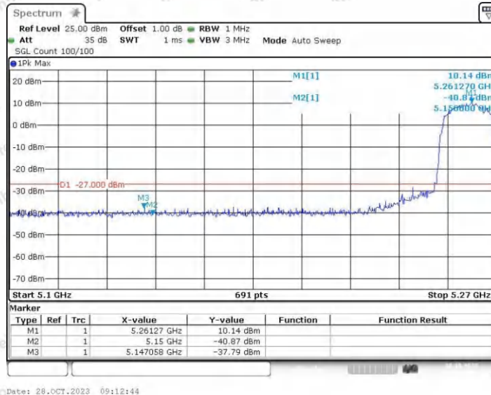
11N20SISO_Ant2_Low_5260
