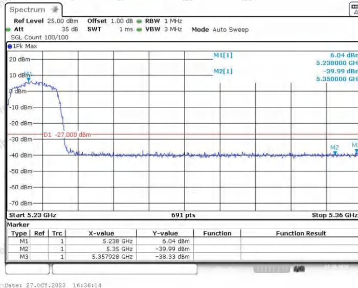
11AC20SISO_Ant1_Low_5260
