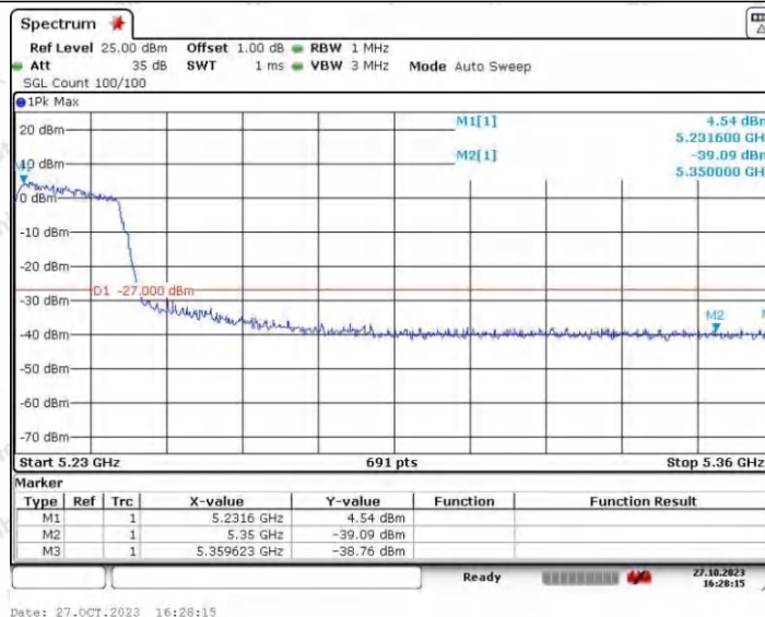
11N40SISO_Ant2_High_5230
