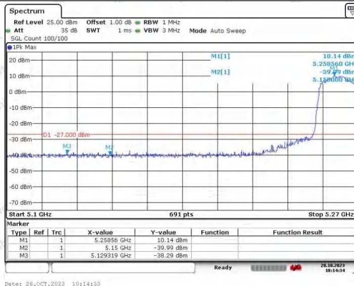
11AC20SISO_Ant2_Low_5260
