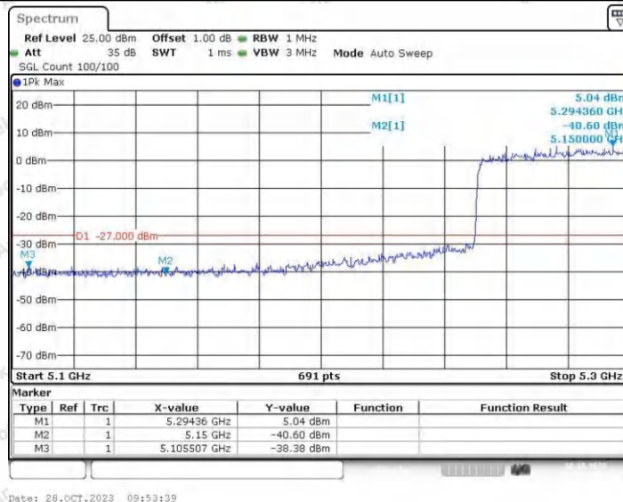
11AX80SISO_Ant2_Low_5290
