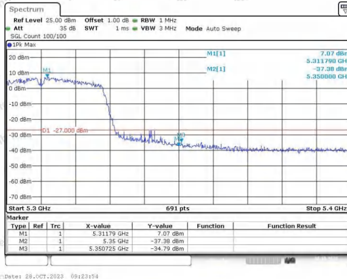
11N40SISO_Ant2_High_5310
