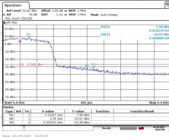
11AC40SISO_Ant2_High_5310
