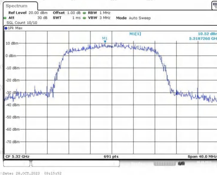
11N20SISO_Ant2_5320
