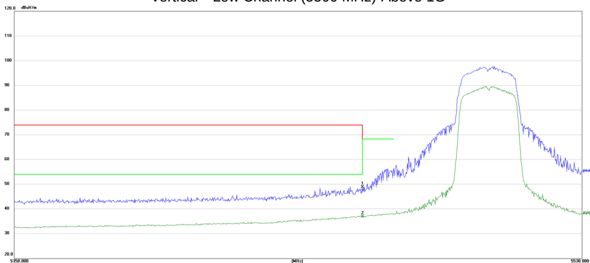
Vertical Low Channel (5500 MHz)-Above 1G
