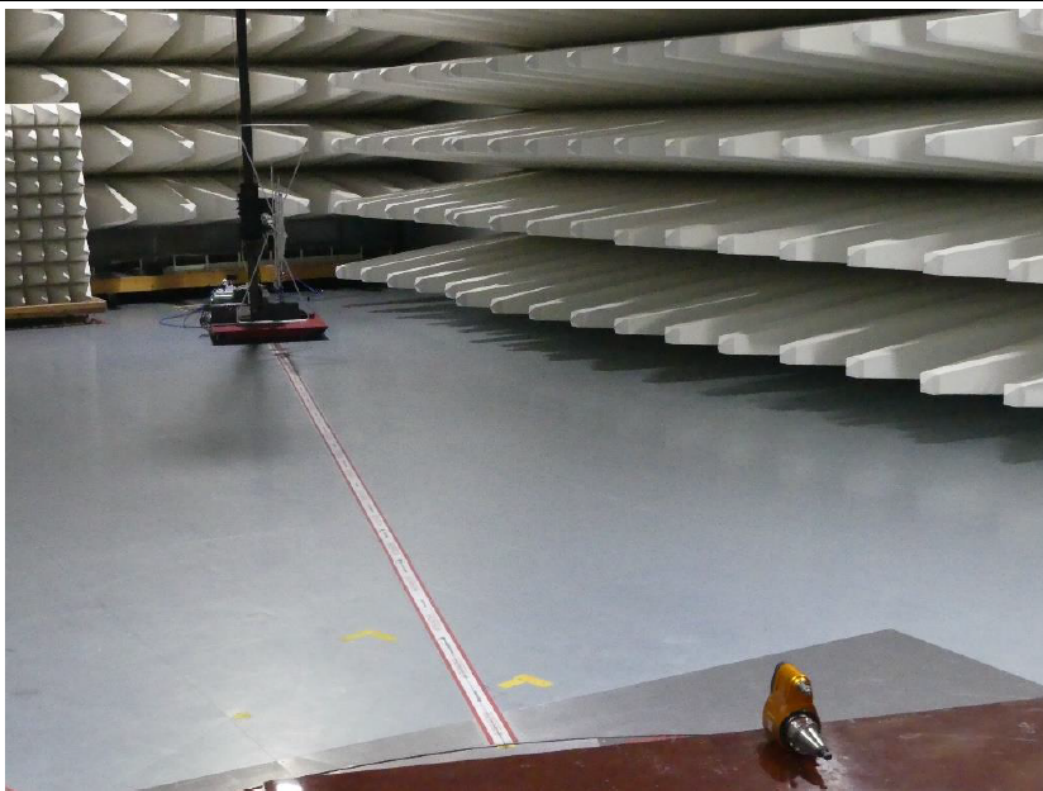
Test setup vertical
