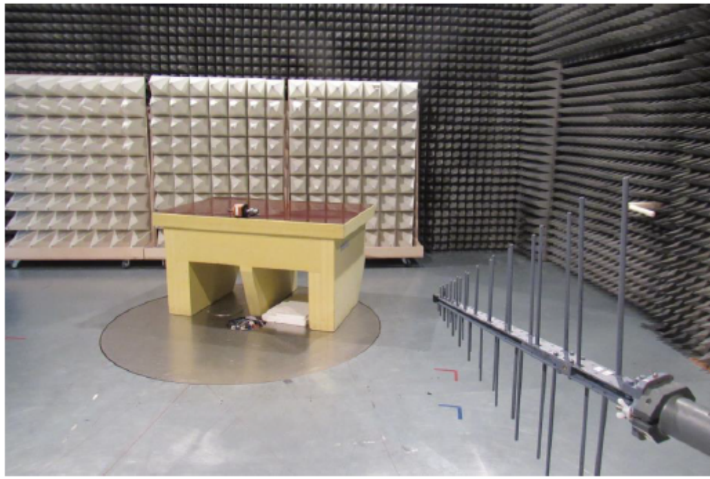
Test setup 200-1000MHz
