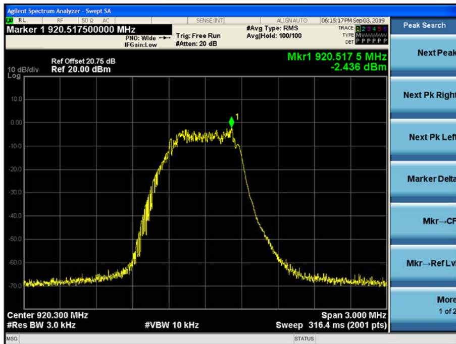
Power Spectral Density (Mid)
