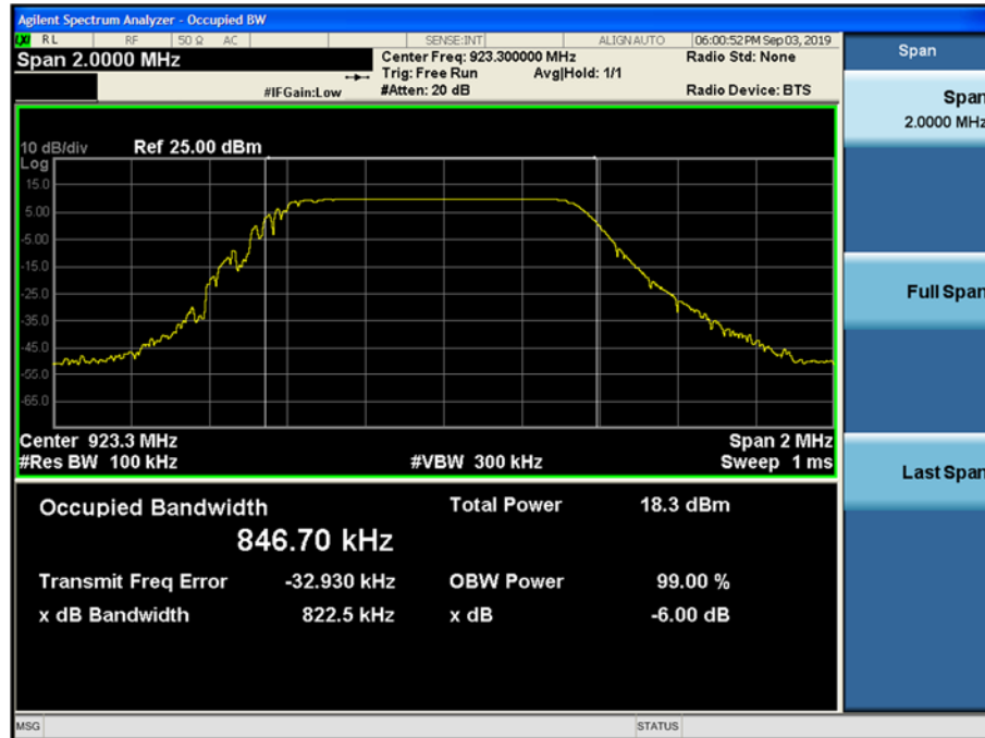
6dB Bandwidth plot (High)
