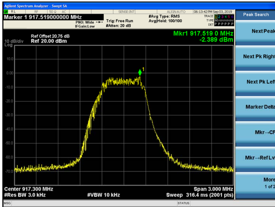
Power Spectral Density (Low)
