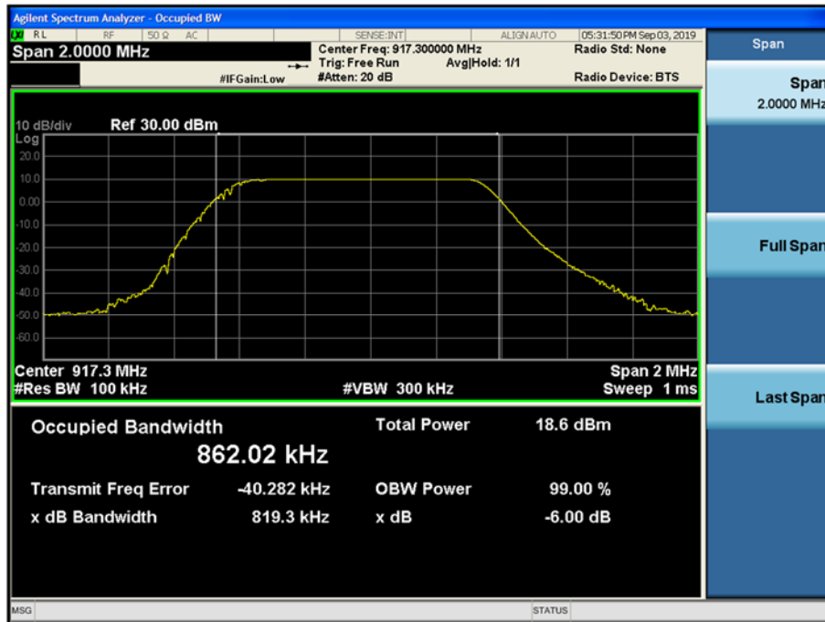
6dB Bandwidth plot (Low)
