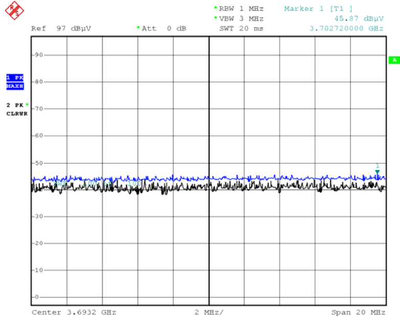
Radiated Spurious Emissions plot – Peak Reading (High 4th Harmonic)
