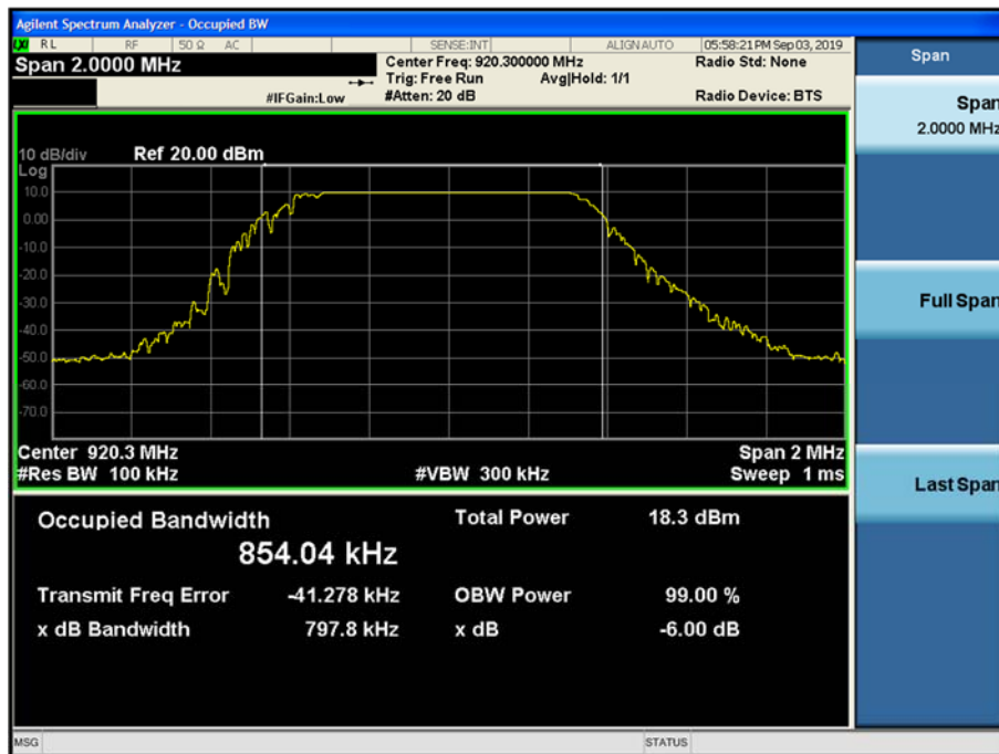
6dB Bandwidth plot (Mid)
