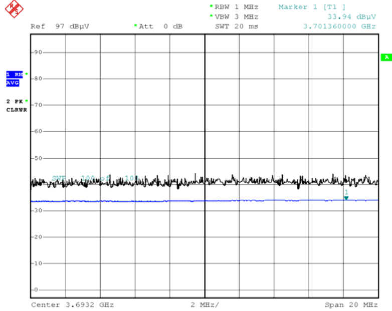
Radiated Spurious Emissions plot – Average Reading (High 4th Harmonic)
