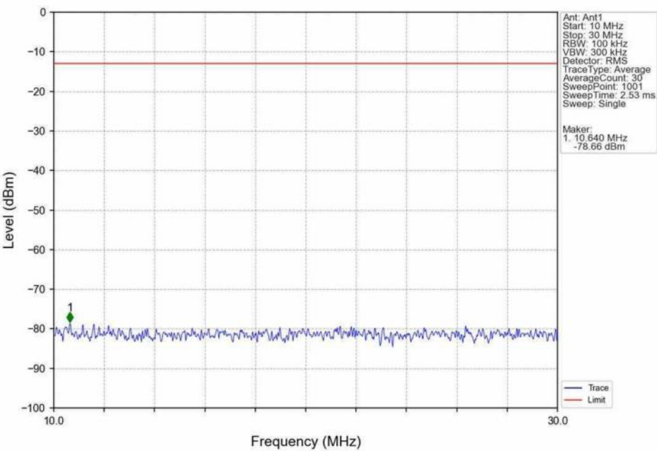
Band12 10MHz 16QAM LCH 704MHz RB 1 0 NTN
