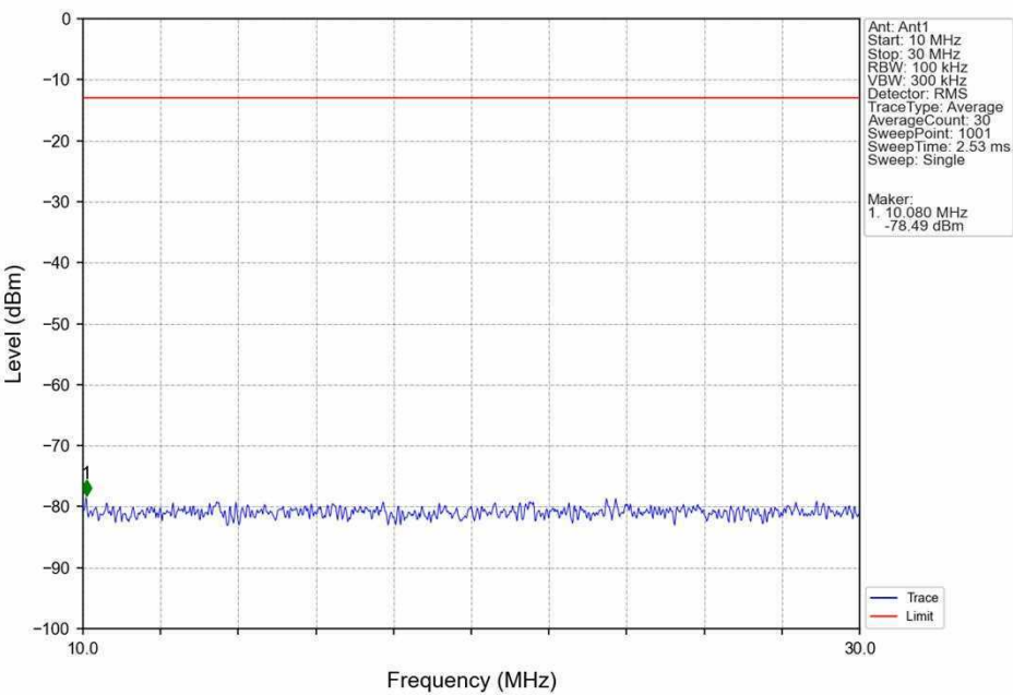
Band12 10MHz QPSK LCH 704MHz RB 1 0 NTV
