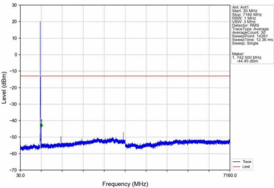
Band12 10MHz 16QAM HCH 711MHz RB 1 49 NTNV
