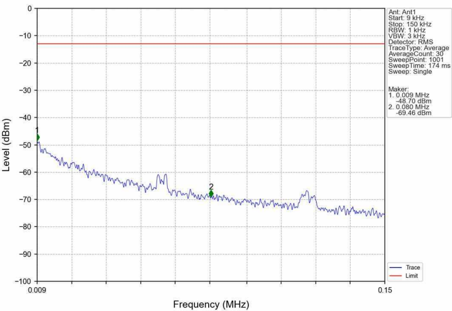
Band12 5MHz QPSK HCH 713.5MHz RB 1 0 NTN
