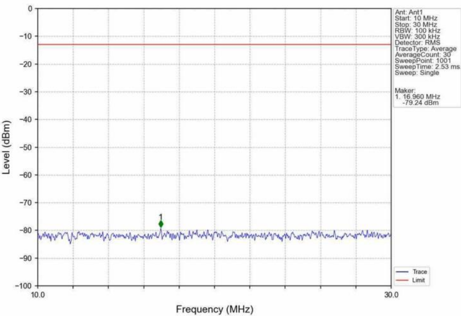
Band12 1.4MHz QPSK HCH 715.3MHz RB 1 0 NTNV
