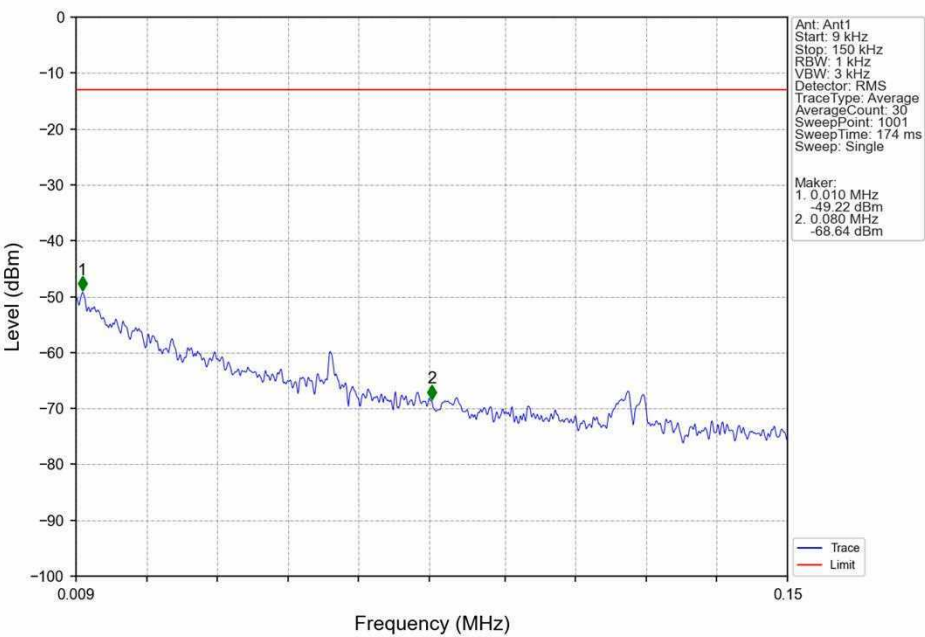
Band12 3MHz QPSK HCH 714.5MHz RB 1 0 NTN
