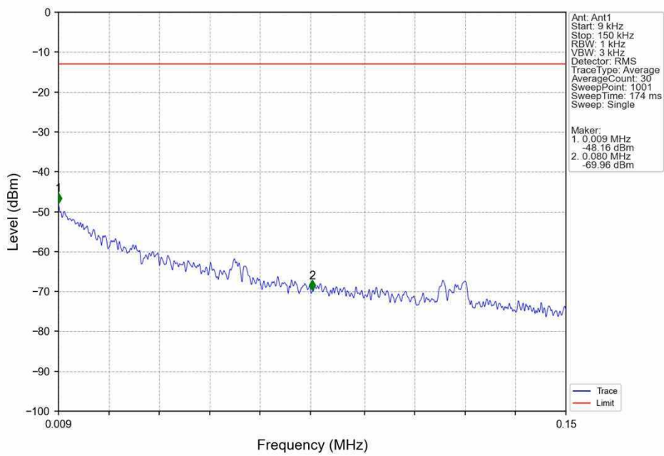
Band4 20MHz 16QAM HCH 1745MHz RB 1 0 NTNV
