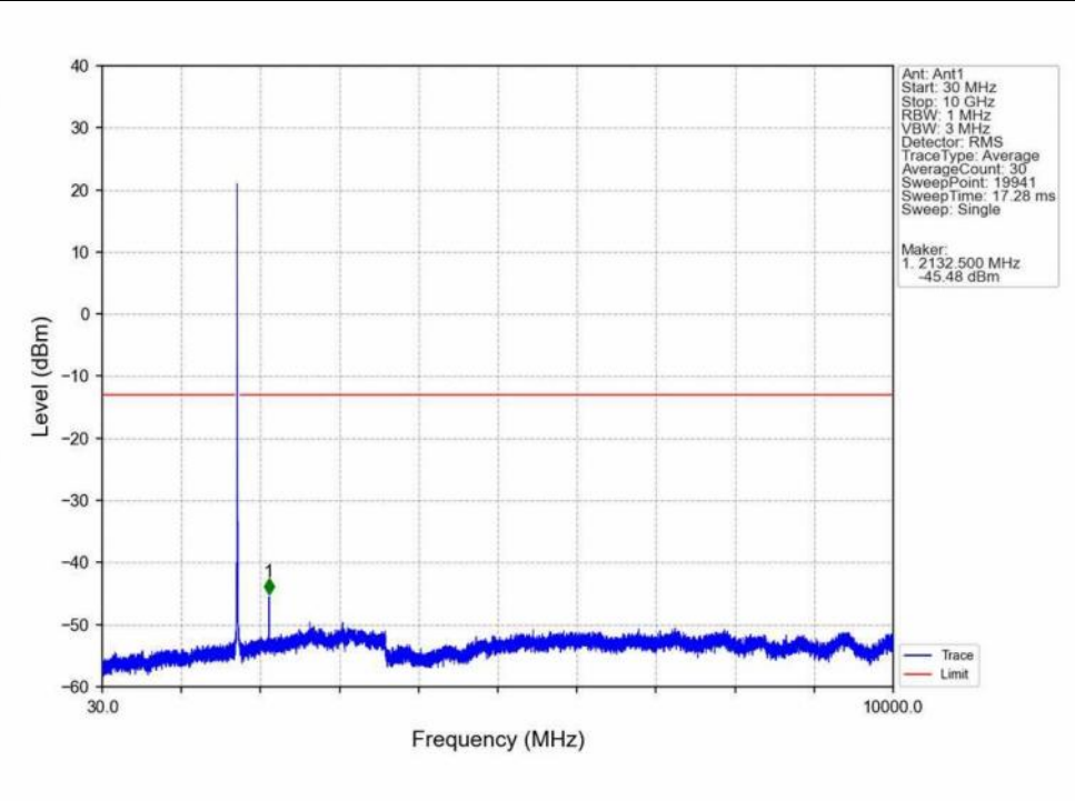
Band4 5MHz 16QAM MCH 1732.5MHz RB 1 0 NTV
