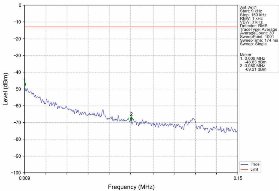
Band4 15MHz QPSK HCH 1747.5MHz RB 1 0 NTV
