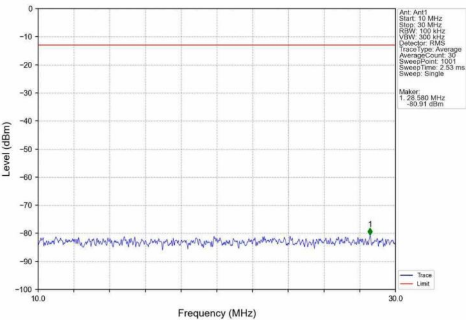
Band4 10MHz 16QAM MCH 1732.5MHz RB 1 0 NTNV
