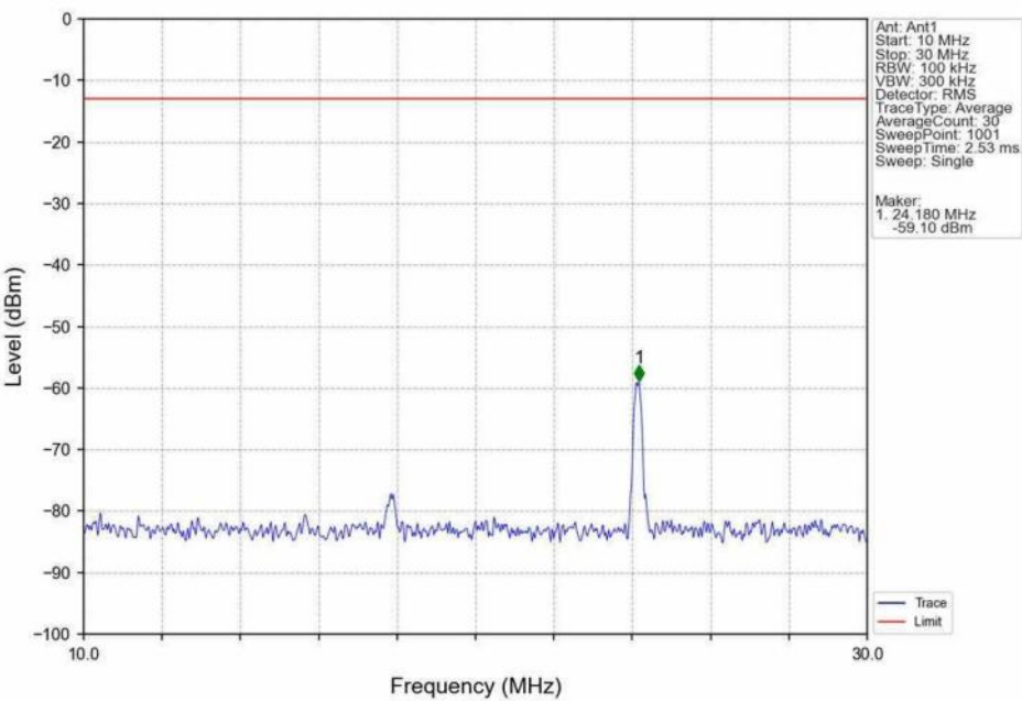
Band4 20MHz 16QAM MCH 1732.5MHz RB 1 0 NTNV
