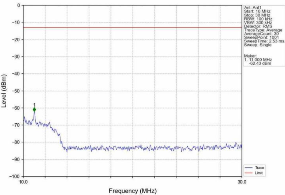
Band4 15MHz 16QAM MCH 1732.5MHz RB 1 0 NTV
