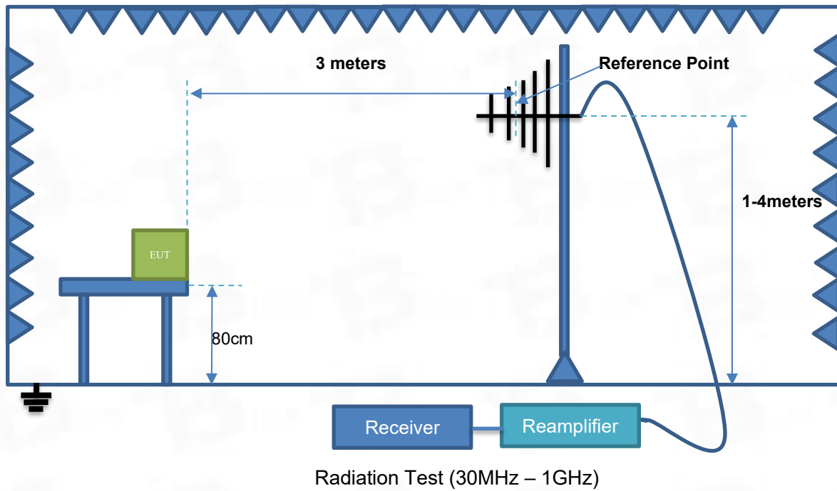
Test Setup 2
