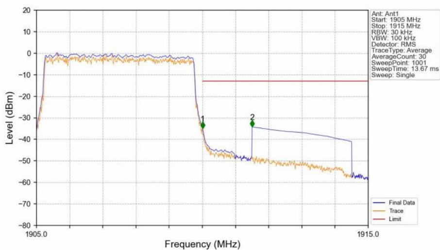
Band2_5MHz_16QAM_HCH_1907.5MHz_RB_25_0_NTNV
