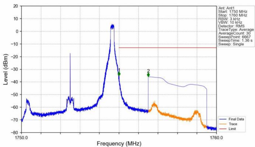
Band4_5MHz_QPSK_HCH_1752.5MHz_RB_1_24_NTNV
