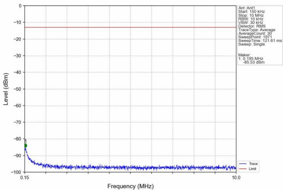
Band4_3MHz_QPSK_HCH_1753.5MHz_RB_1_0_NTNV
