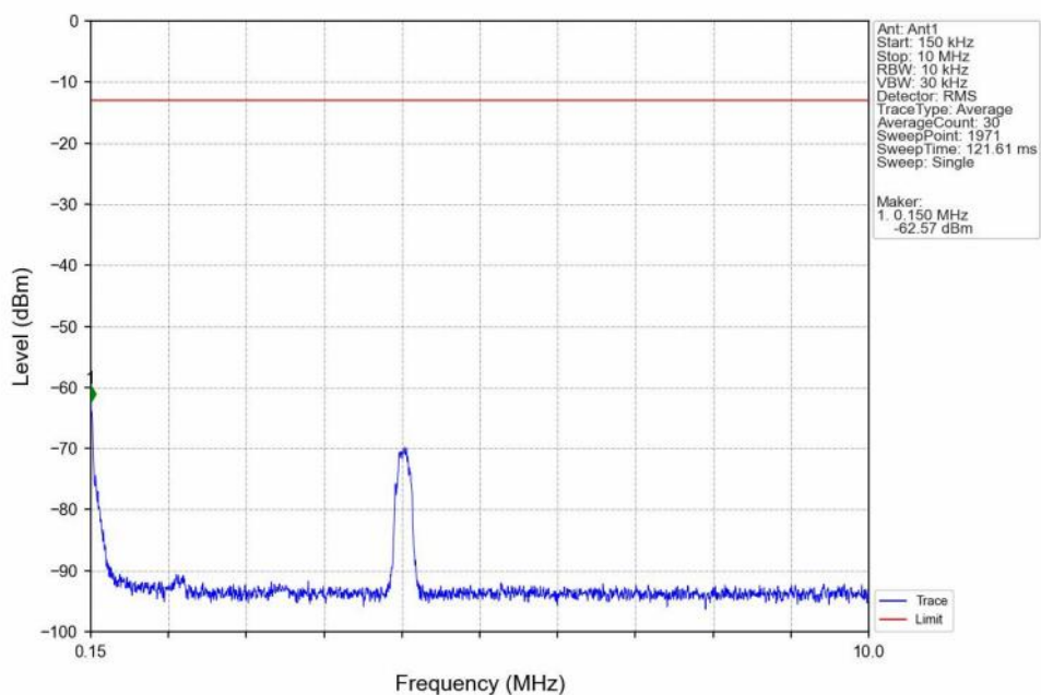
Band4_3MHz_16QAM_LCH_1711.5MHz_RB_1_0_NTNV
