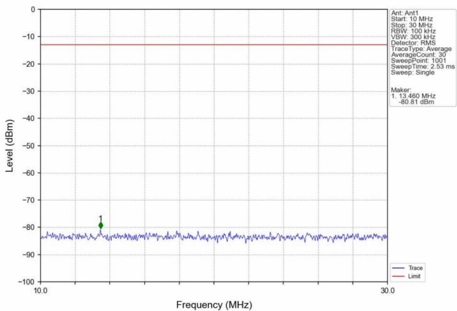
Band4_10MHz_QPSK_LCH_1715MHz_RB_1_0_NTNV
