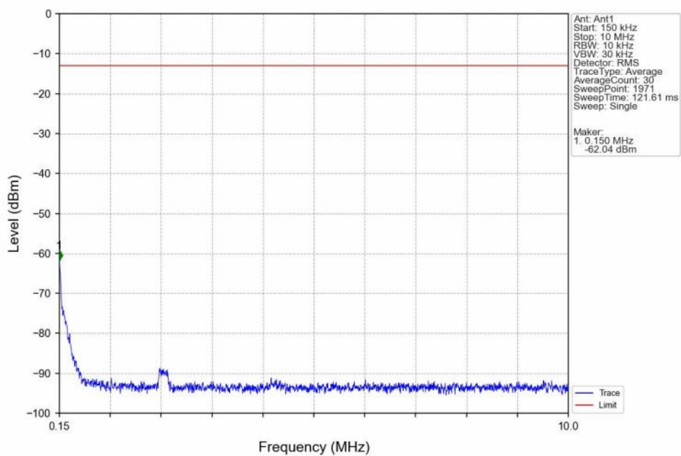
Band4_5MHz_QPSK_HCH_1752.5MHz_RB_1_0_NTNV
