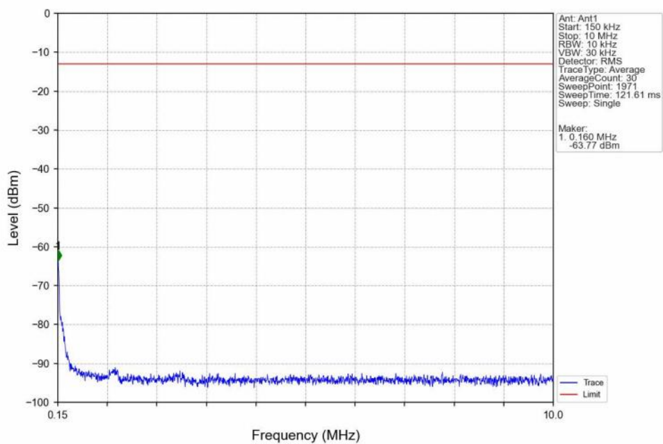
Band4_3MHz_16QAM_MCH_1732.5MHz_RB_1_0_NTNV
