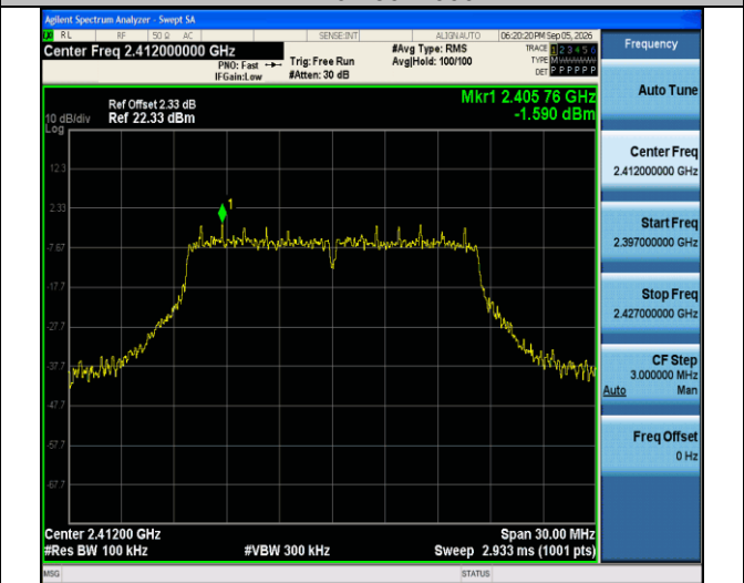
11g-Ant1-2412-0~Reference-PASS
