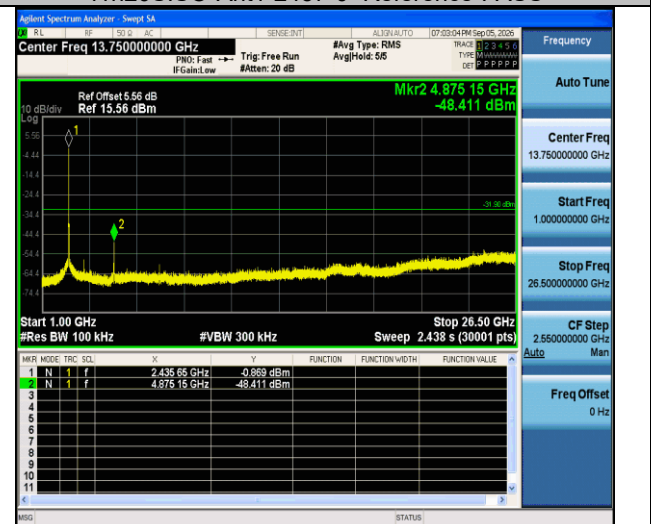
11n20SISO-Ant1-2437-1000~26500-PASS
