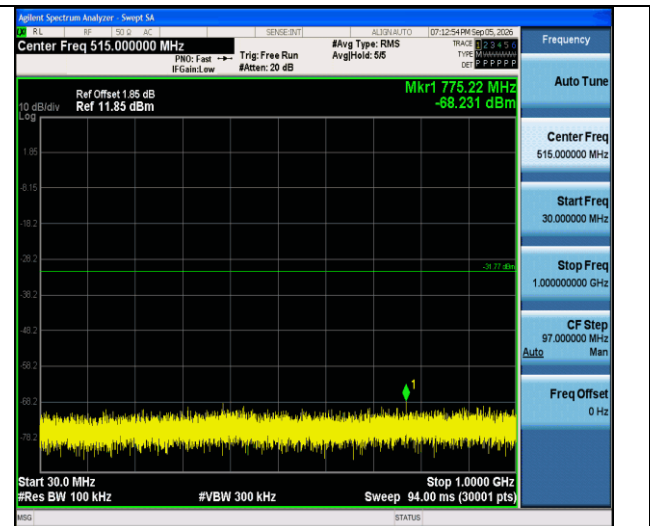
11n20SISO-Ant1-2462-30~1000-PASS
