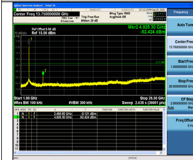
11n20SISO-Ant1-2462-1000~26500-PASS
