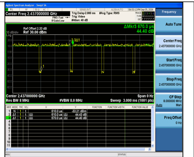
NTNV-11n20SISO-Ant1-2437
