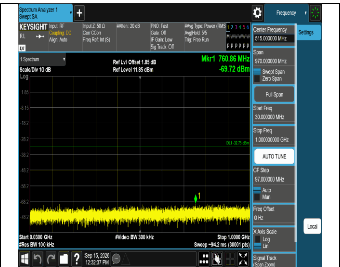
11b-Ant1-2462-30~1000-PASS
