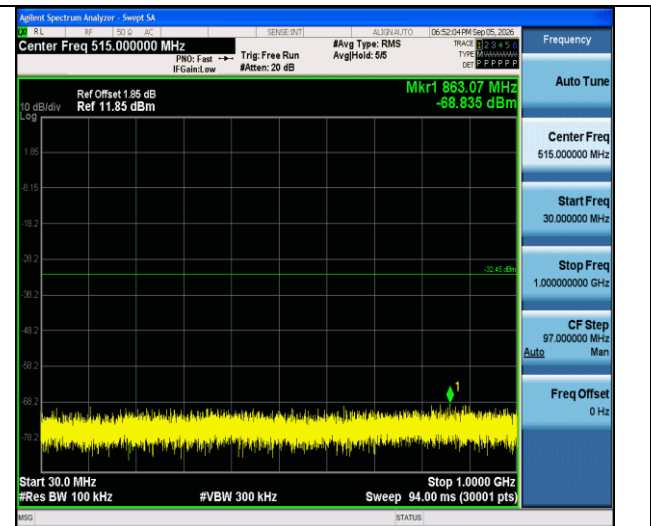
11n20SISO-Ant1-2412-30~1000-PASS
