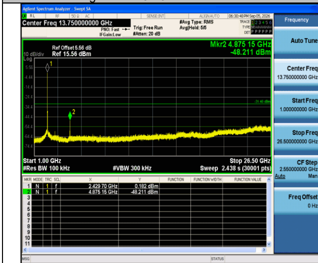
11g-Ant1-2437-1000~26500-PASS
