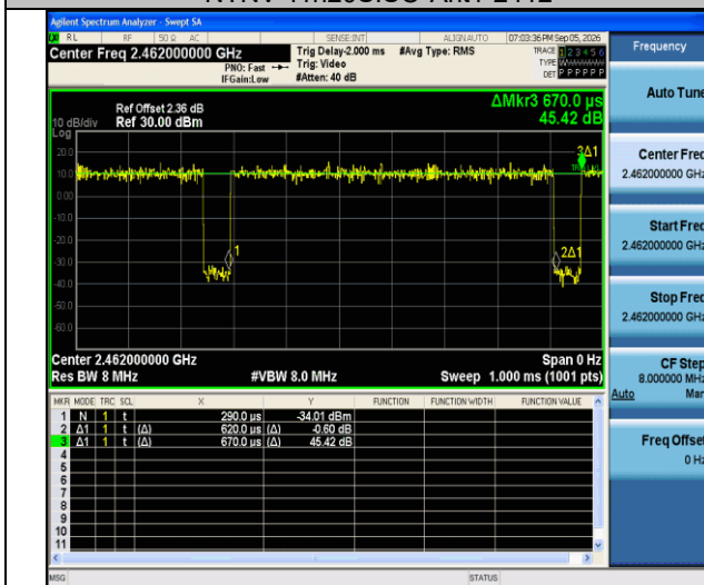
NTNV-11n20SISO-Ant1-2462
