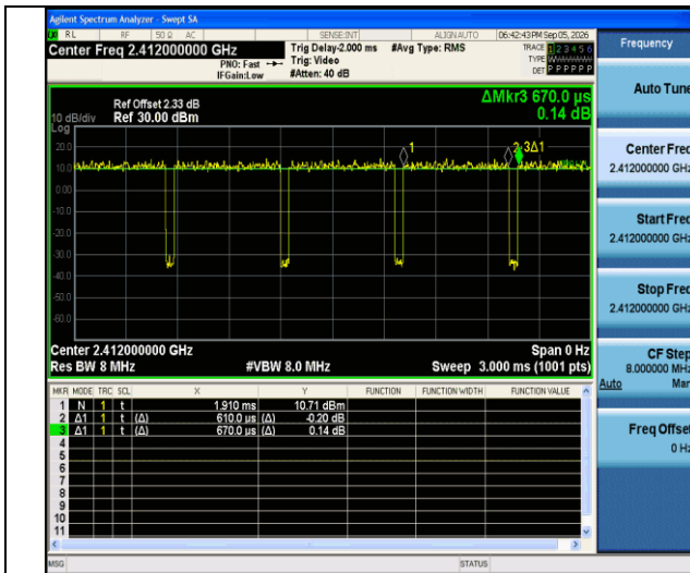
NTNV-11n20SISO-Ant1-2412
