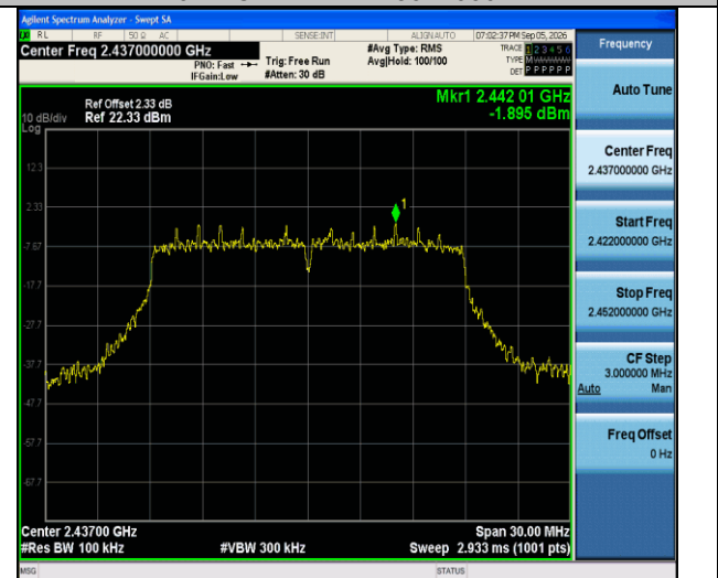
11n20SISO-Ant1-2437-0~Reference-PASS
