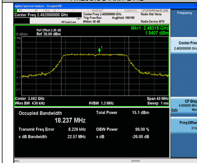
11n20SISO-Ant1-2462
