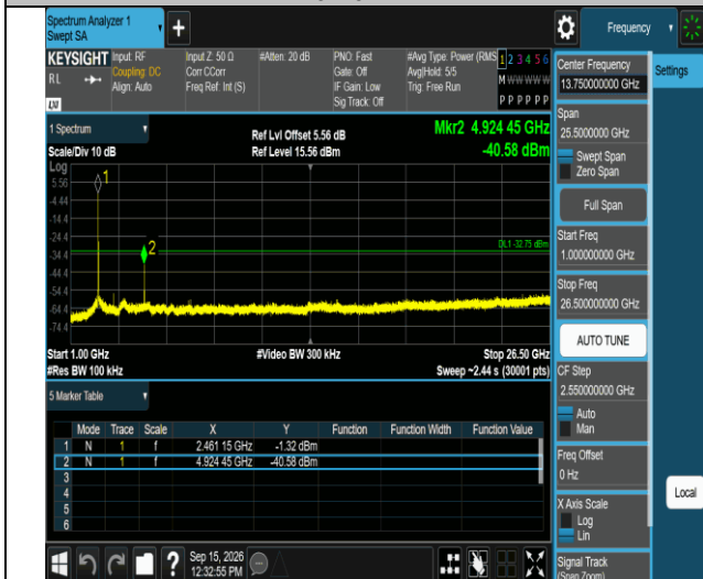
11b-Ant1-2462-1000~26500-PASS
