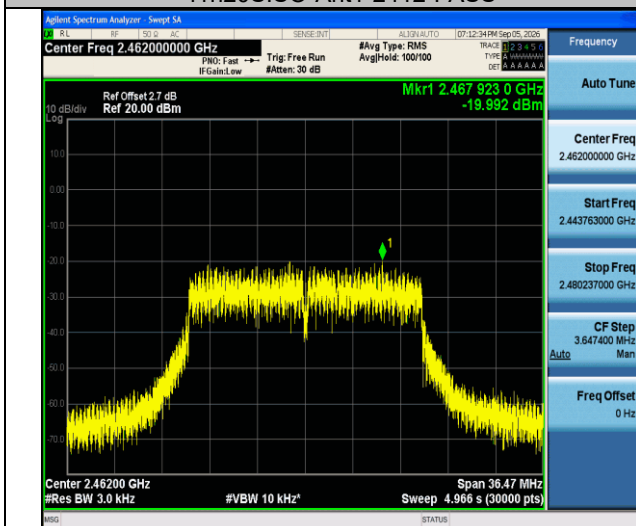
11n20SISO-Ant1-2462-PASS
