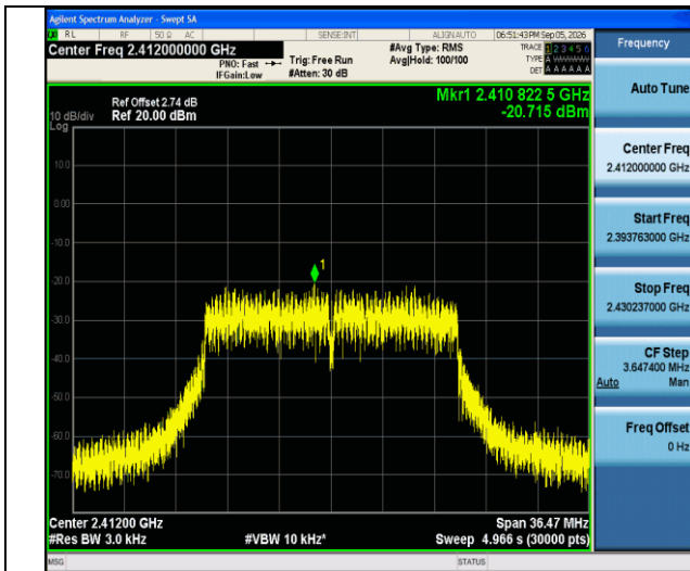
11n20SISO-Ant1-2412-PASS
