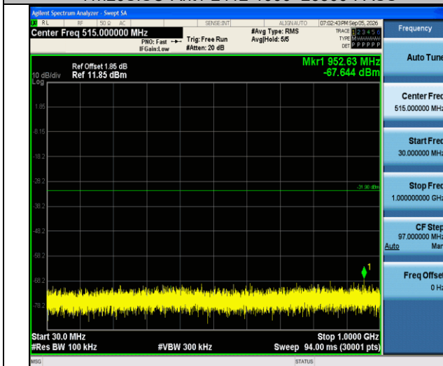
11n20SISO-Ant1-2437-30~1000-PASS
