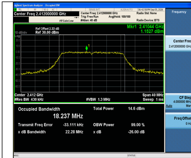
11n20SISO-Ant1-2412
