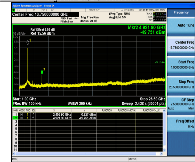
11g-Ant1-2462-1000~26500-PASS
