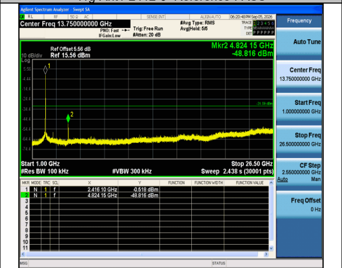
11g-Ant1-2412-1000~26500-PASS
