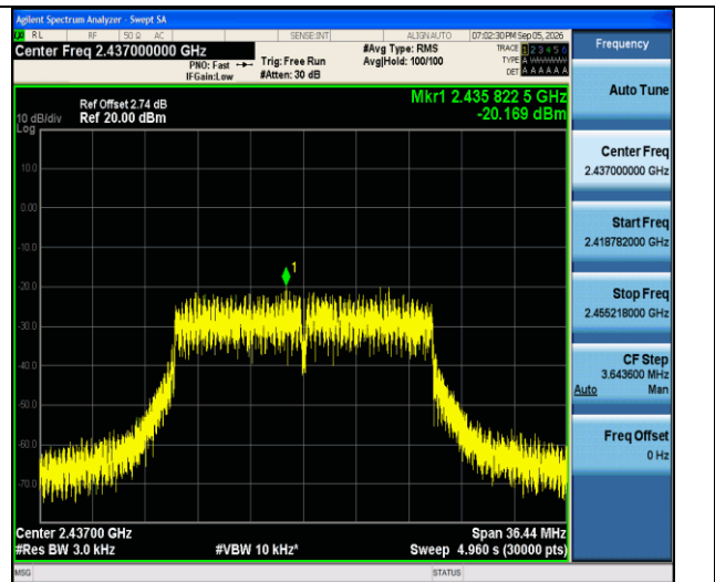
11n20SISO-Ant1-2437-PASS
