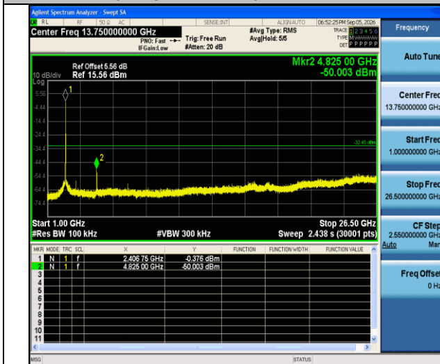
11n20SISO-Ant1-2412-1000~26500-PASS
