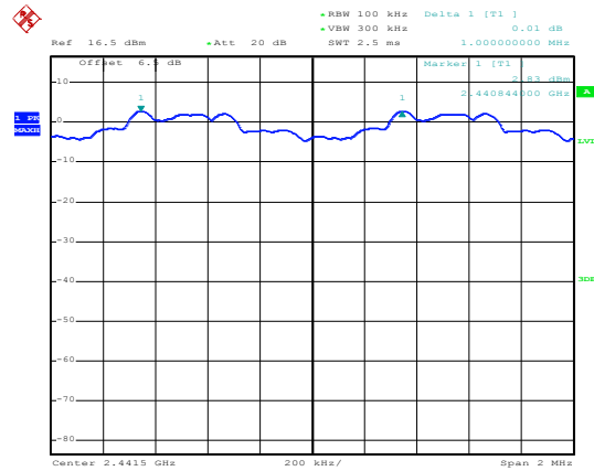
Modulation mode:8DPSK
