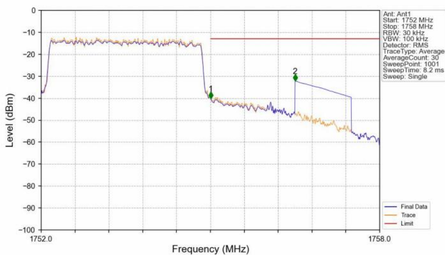
Band4_3MHz_16QAM_HCH_1753.5MHz_RB_15_0_NTNV
