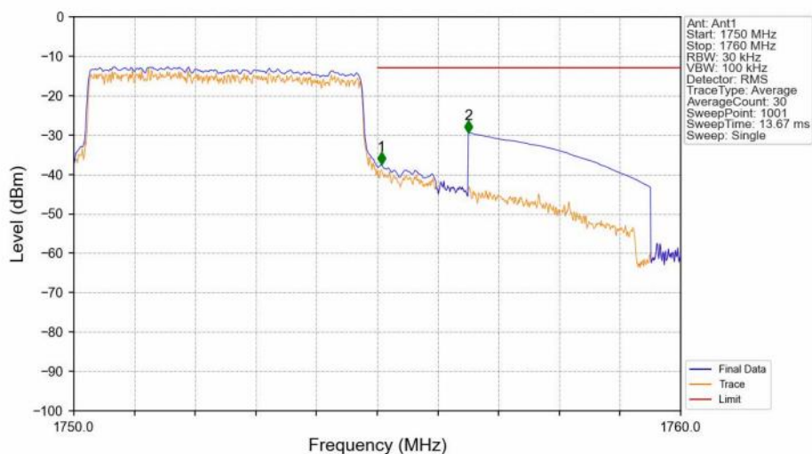
Band4_5MHz_QPSK_HCH_1752.5MHz_RB_25_0_NTNV
