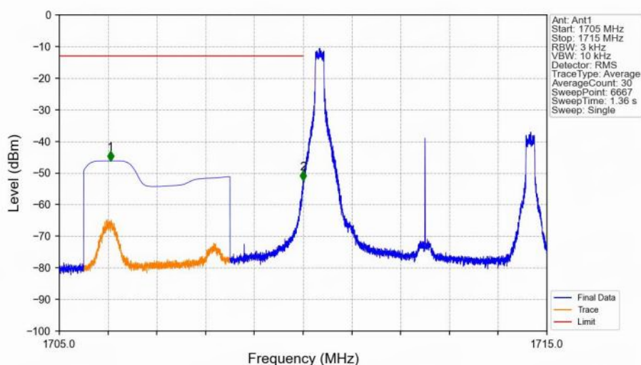
Band4_5MHz_16QAM_LCH_1712.5MHz_RB_1_0_NTNV
