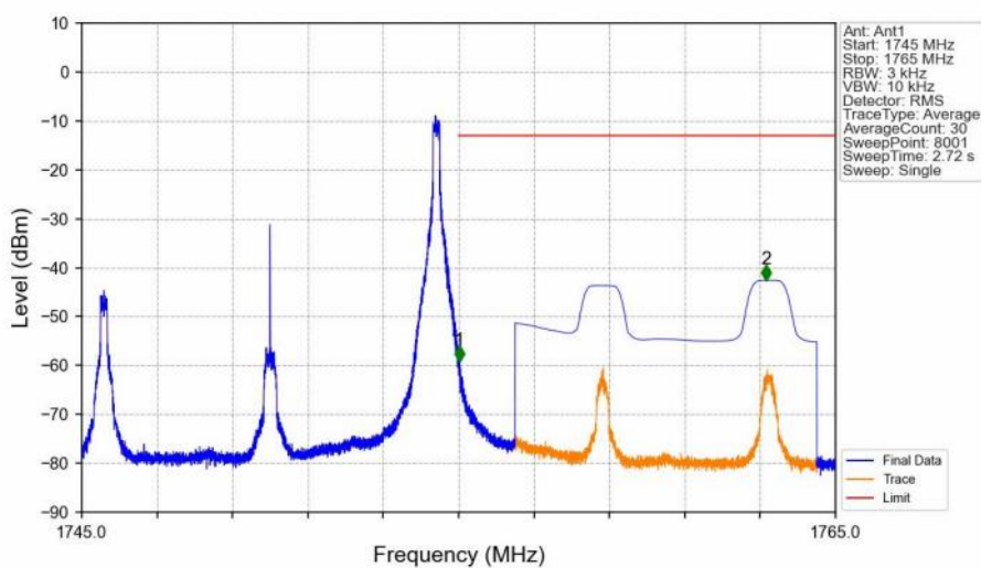
Band4_10MHz_16QAM_HCH_1750MHz_RB_1_49_NTNV
