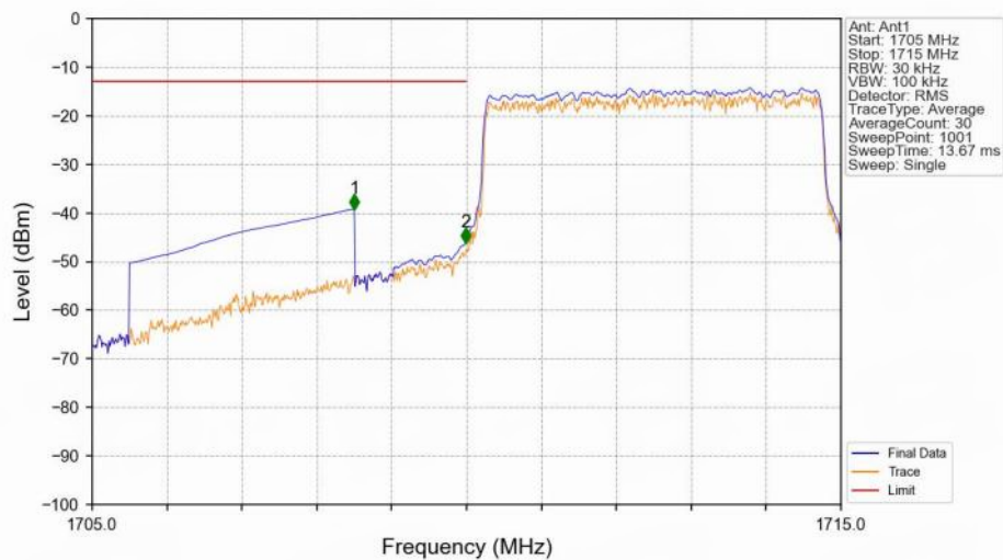
Band4_5MHz_16QAM_LCH_1712.5MHz_RB_25_0_NTNV
