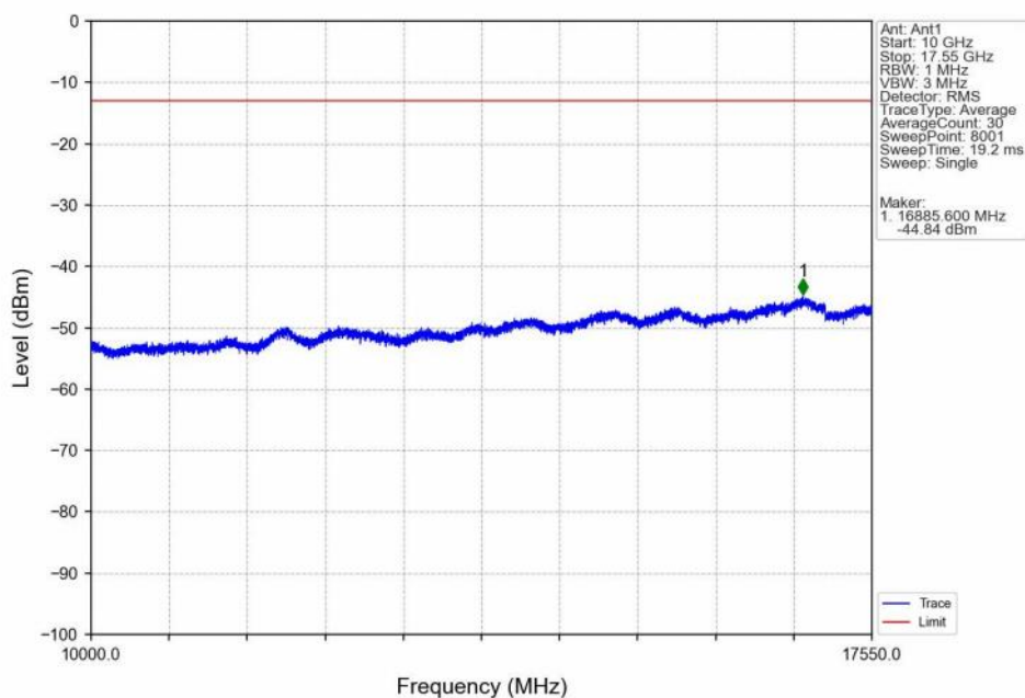
Band4_10MHz_16QAM_HCH_1750MHz_RB_1_49_NTNV
