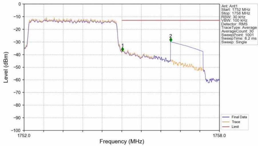
Band4_3MHz_QPSK_HCH_1753.5MHz_RB_15_0_NTNV
