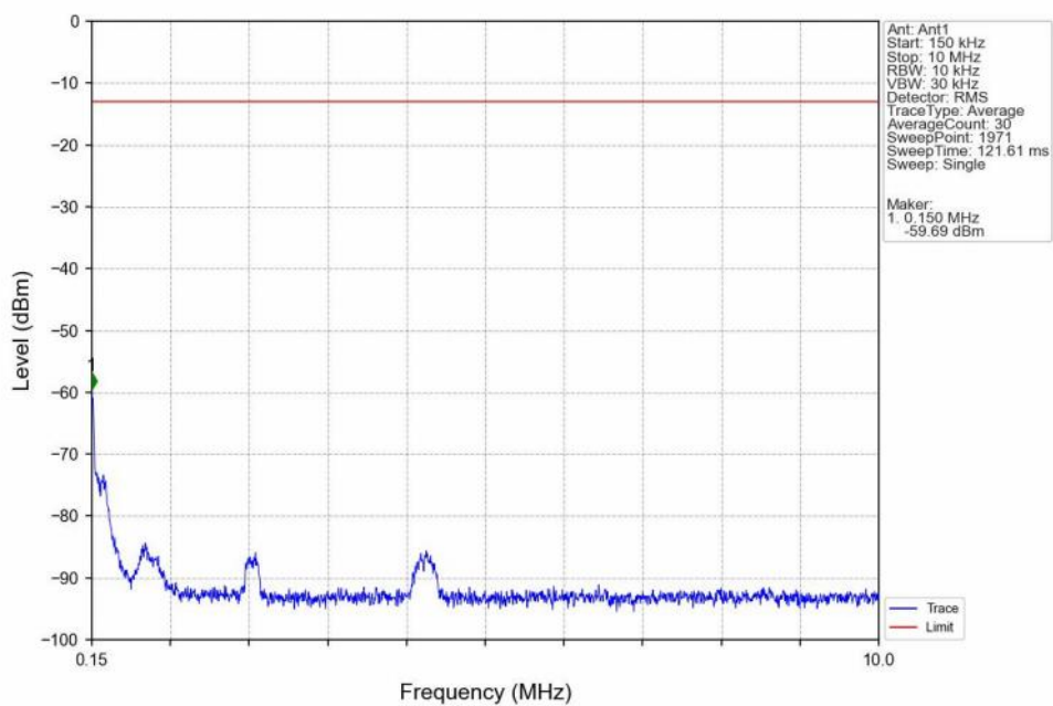
Band4_5MHz_16QAM_MCH_1732.5MHz_RB_1_0_NTNV
