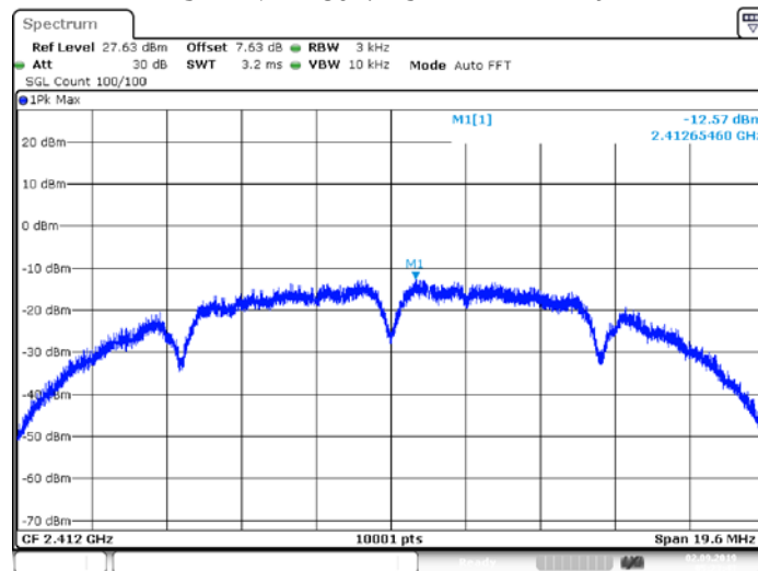
PSD NVNT 802.11b 2412MHz Ant1
