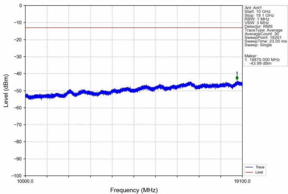
Band2_5MHz_QPSK_HCH_1907.5MHz_RB_1_24_NTNV
