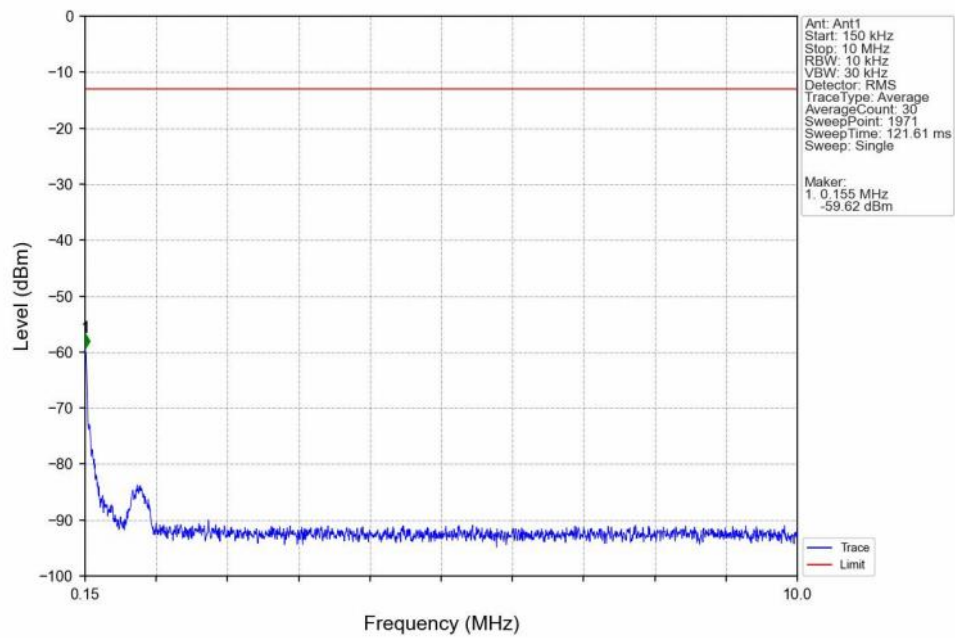
Band2_1.4MHz_16QAM_LCH_1850.7MHz_RB_1_0_NTNV
