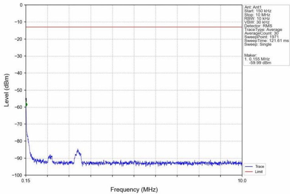
Band2_3MHz_16QAM_LCH_1851.5MHz_RB_1_0_NTNV
