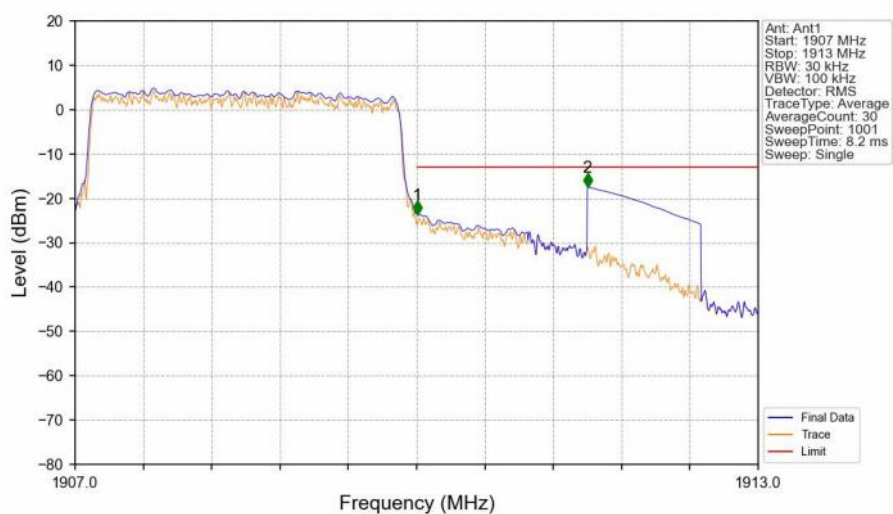
Band2_3MHz_16QAM_HCH_1908.5MHz_RB_15_0_NTNV
