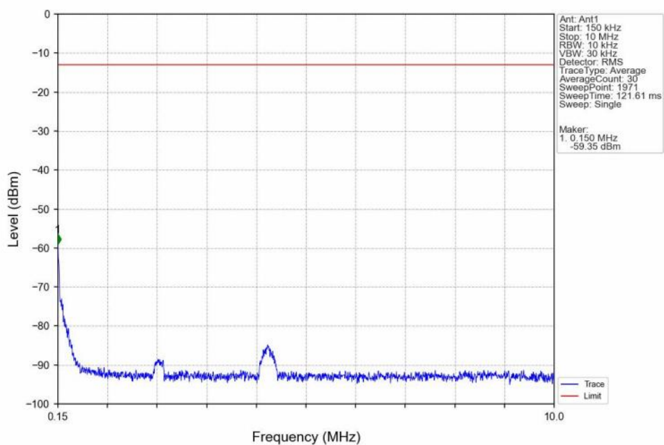
Band2_5MHz_16QAM_LCH_1852.5MHz_RB_1_0_NTNV
