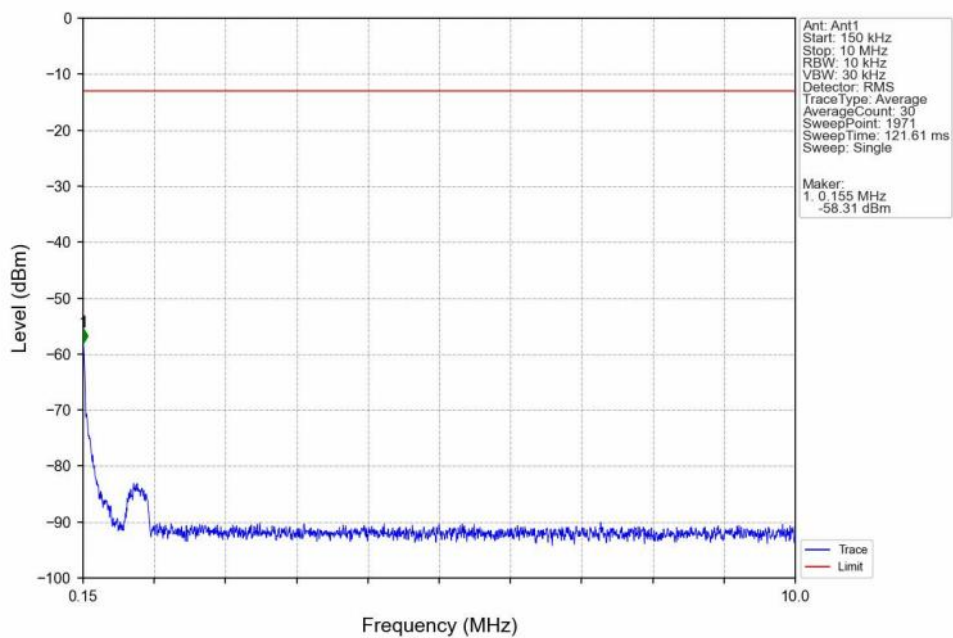
Band2_1.4MHz_QPSK_LCH_1850.7MHz_RB_1_0_NTNV
