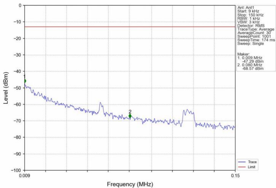
Band2_5MHz_16QAM_LCH_1852.5MHz_RB_1_0_NTNV
