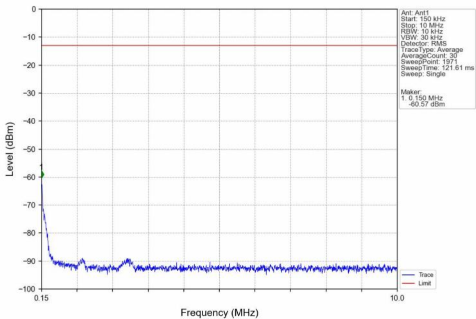
Band2_3MHz_16QAM_HCH_1908.5MHz_RB_1_0_NTNV
